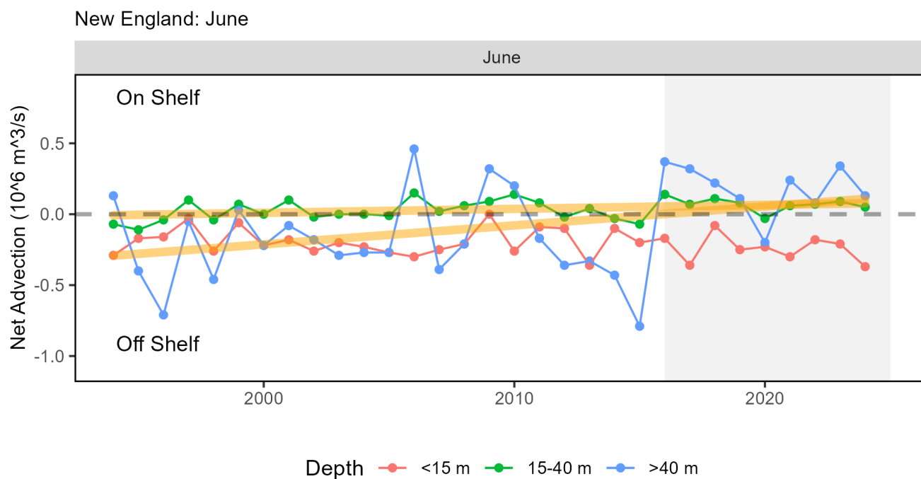
Figure 59: Net advection in June across the Southern New England and Georges Bank continental shelf break within 3 depth bands.
