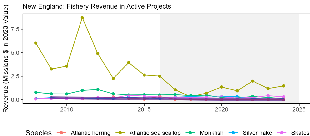
Figure 63: Revenue of species managed by the New England Fishery Management Council within existing offshore wind lease areas.
