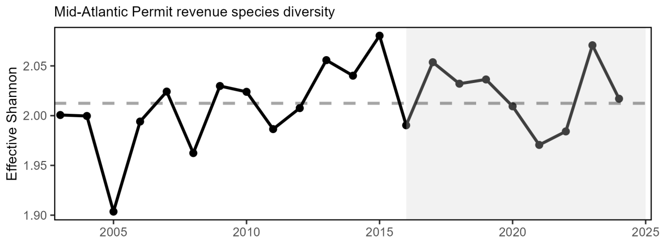
Figure 26: Species revenue diversity (permit-level species effective Shannon index) in the Mid-Atlantic.
