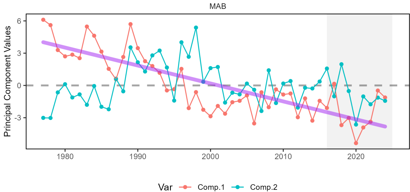
Figure 30: Principal component analysis of zooplankton community composition in the Mid-Atlantic Bight. Lines show the first two principal components (colors). The long-term declining trendline (purple) is associated with the first principal component. This trend is driven by an increasing abundance of sea butterflies, hyperiid amphipods, echinoderm larvae, arrow worms, and the copepod Calanus minor , and a decreasing abundance of the copepods Pseudocalanus spp. , Centropages hamatus , Acartia spp. , and Temora longicornis .
