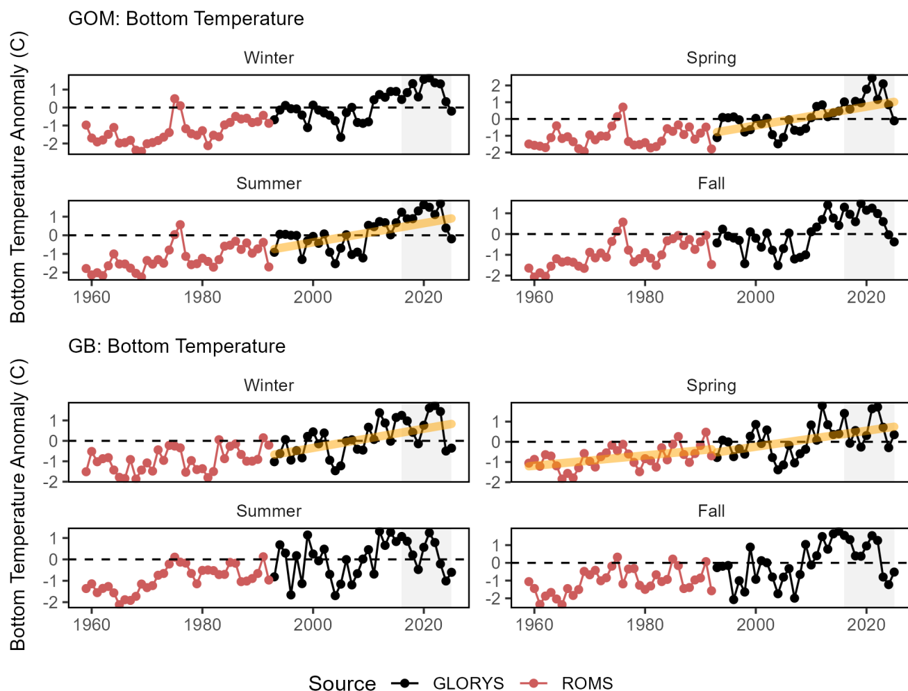
Figure 44: GLORYS (black) and debiased Regional Ocean Modeling System (ROMS) (red) seasonal bottom temperature anomaly for the Gulf of Maine (GOM, top) and Georges Bank (GB, bottom), with long-term increasing trends (orange).
