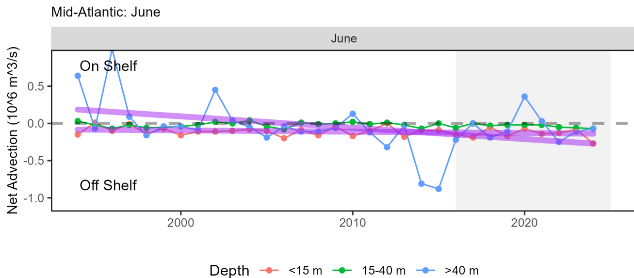
Figure 56: Net advection in June across the Mid-Atlantic continental shelf break within 3 depth bands.
