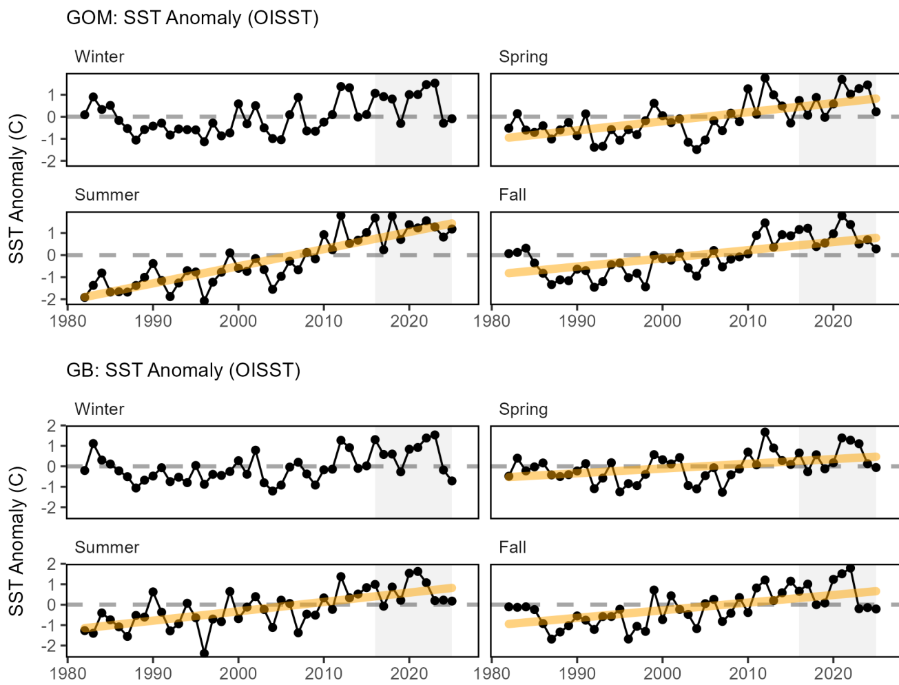
Figure 41: Seasonal Optimum Interpolation Sea Surface Temperature (OISST) anomaly by season for the GOM (top) and GB (bottom), with long-term increasing trends (orange).
