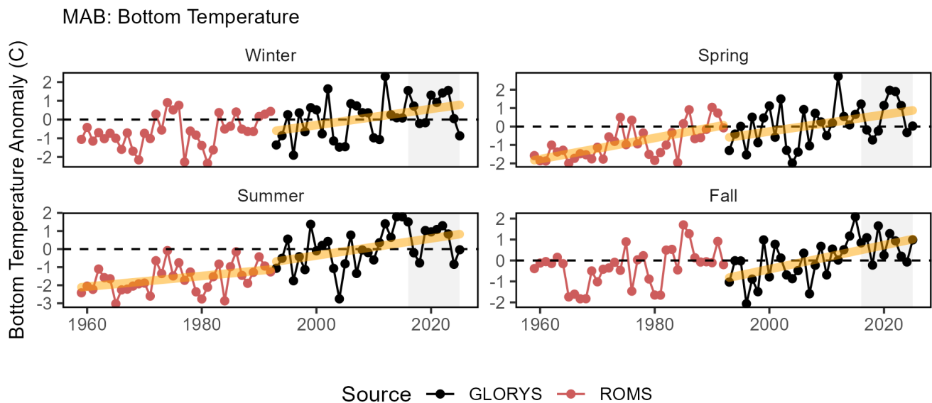
Figure 42: GLORYS (black) and debiased ROMS (red) seasonal bottom temperature anomaly in the MAB, with long-term increasing trends (orange).
