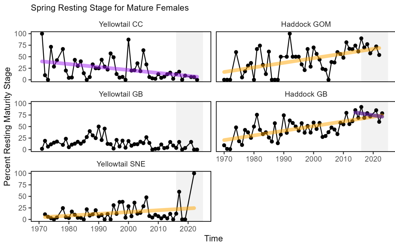
Figure 46: Percent resting stage (non-spawning) mature female fish (black) from spring NEFSC bottom trawl survey with significant long-term increases (orange), short-term decreases (dark purple), and long-term decreases (purple) from two haddock and three yellowtail flounder stocks: CC = Cape Cod, Gulf of Maine, GOM = Gulf of Maine, GB = Georges Bank, SNE = Southern New England.
