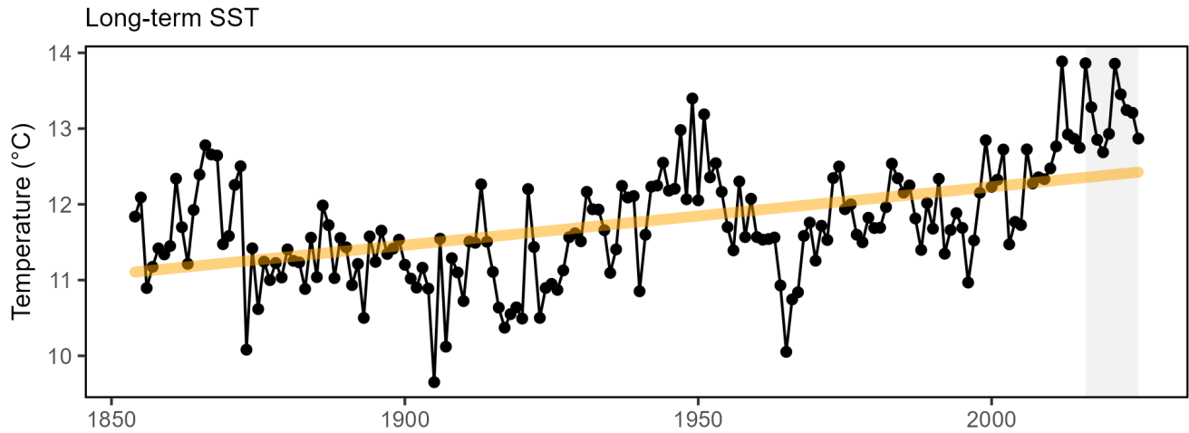
Figure 43: Northeast U.S. annual sea surface temperature (SST, black), with long-term increasing trend (orange).
