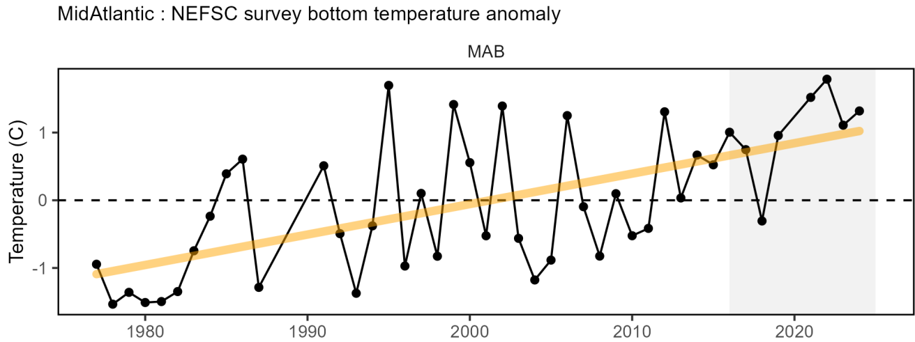
Figure 41: Annual in situ bottom temperature anomaly in the Mid-Atlantic, with long-term increasing trends (orange).
