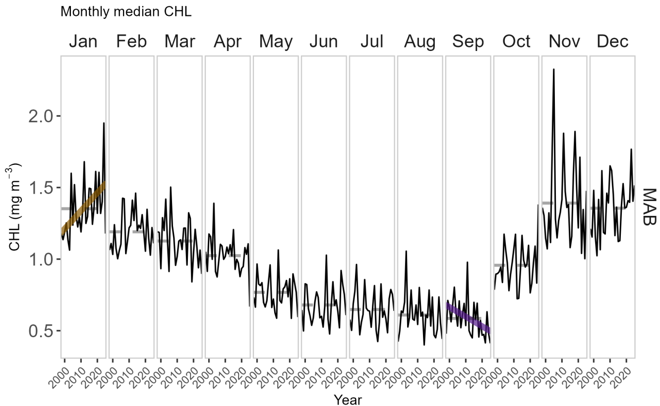
Figure 49: Monthly median chlorophyll a concentration in the MAB (black) with a significant long-term increase present in January (orange) and a significant long-term decline in September (purple).
