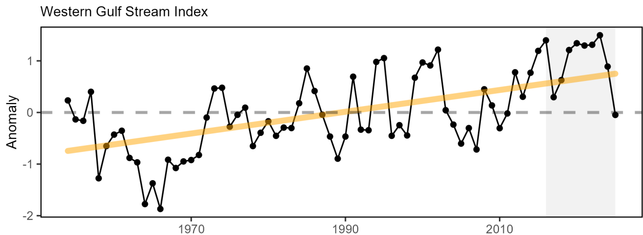
Figure 44: Index representing changes in the location of the western (between 64 and 55 degrees W) Gulf Stream north wall (black). Positive values represent a more northerly Gulf Stream position, with long-term increasing trend (orange).
