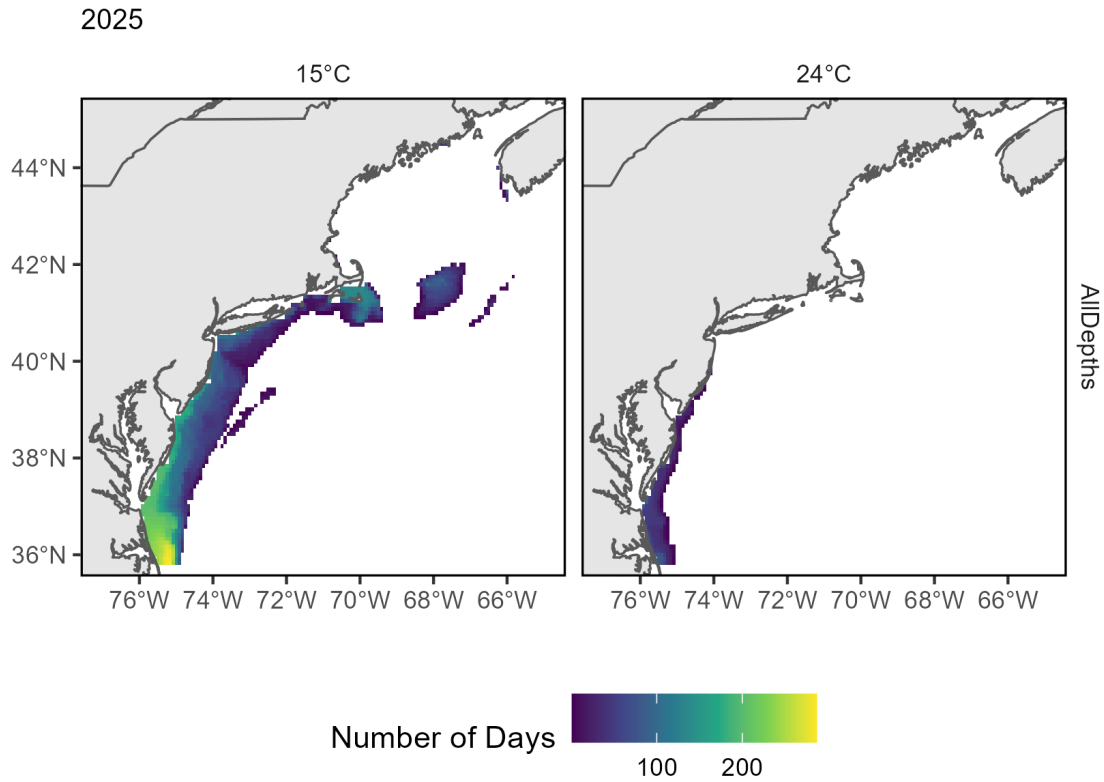
Figure 57: The number of days in 2025 where bottom temperature exceeds 15 degrees (left) and 24 degrees (right) based on the GLORYS 1/12 degree grid.
