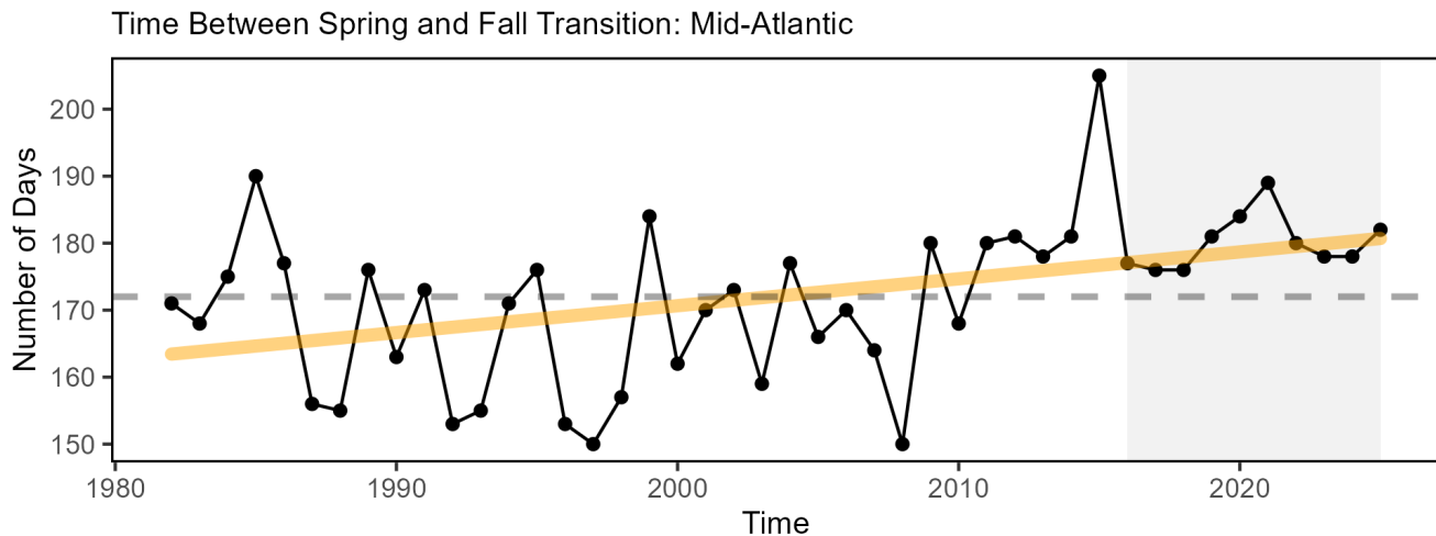
Figure 47: Ocean summer length in the MAB: the annual total number of days between the spring thermal transition date and the fall thermal transition date (black), with a long-term increasing trend (orange). Transition dates are based on sea surface temperatures.
