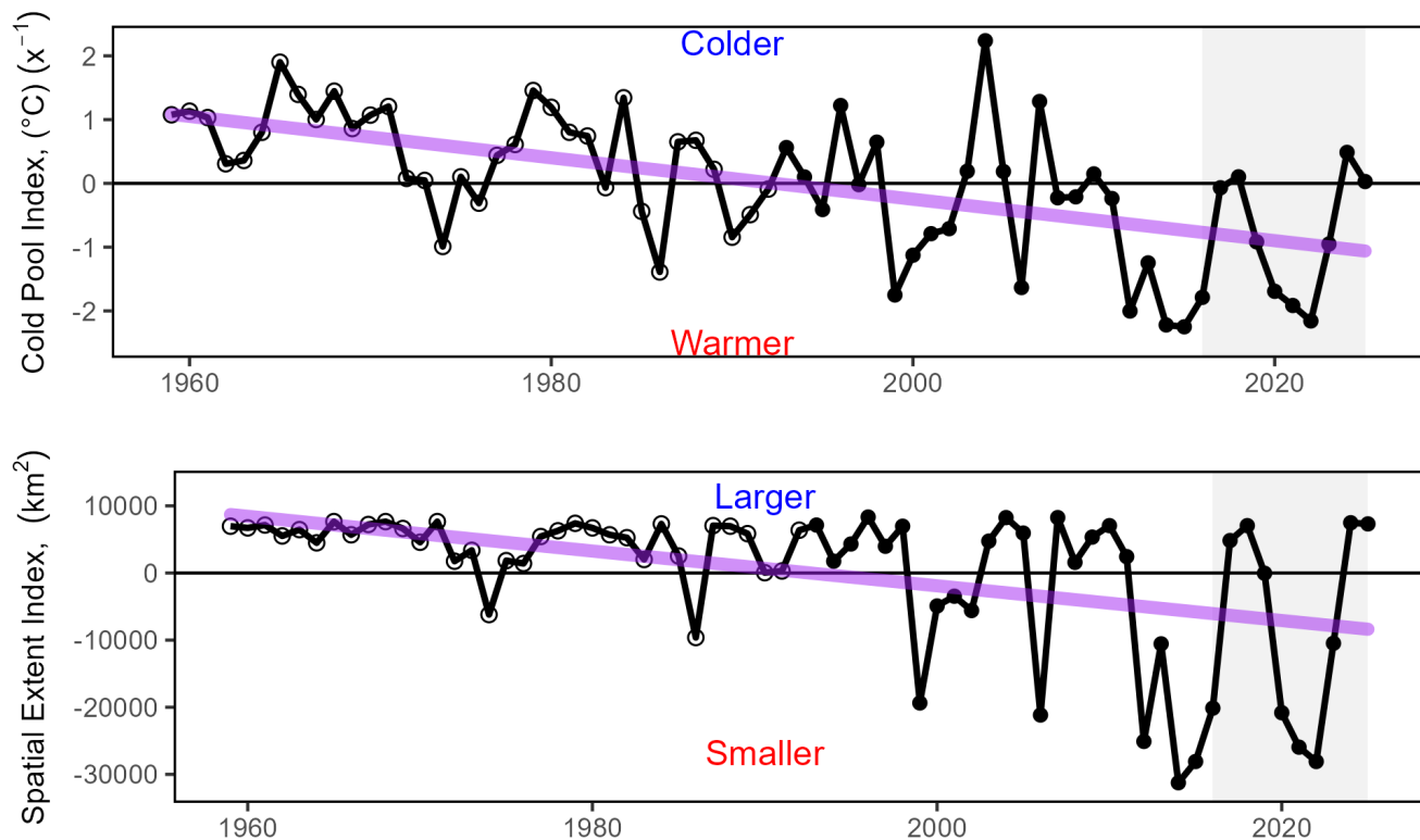
Figure 45: Seasonal cold pool mean temperature (top) and spatial extent index (bottom), based on bias-corrected ROMS-NWA (open circles) and GLORYS (closed circles), with long-term declining trends (purple).
