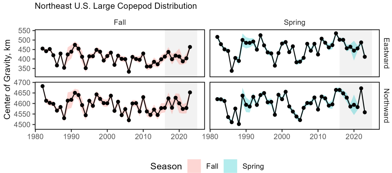
Figure 37: Eastward (top) and northward (bottom) shifts in the center of gravity for large copepod species (( Calanus finmarchicus ), ( Metridia lucens ), ( Calanus minor ), ( Eucalanus sp. ), ( Calanus spp. )) on the Northeast U.S. Shelf in fall (left) and spring (right).
