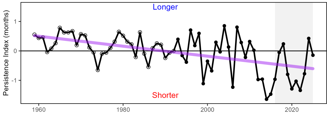
Figure 48: The Mid-Atlantic Bight Cold Pool persistence index based on bias-corrected ROMS-NWA (open circles) and GLORYS (closed circles), with significant long-term decline (purple).
