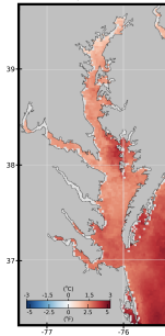
Surface Temperature Difference April 2025
