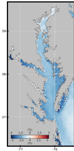
Surface Temperature Difference January 2025
