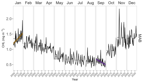
Monthly median CHL
