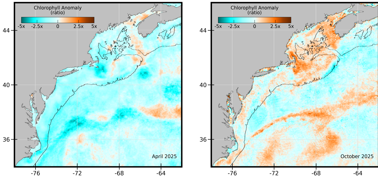
Figure 73: Chlorophyll anomalies shown as the ratio of the monthly concentration compared to the climatological mean (1998-2020) for April (left) and October (right), 2025.
