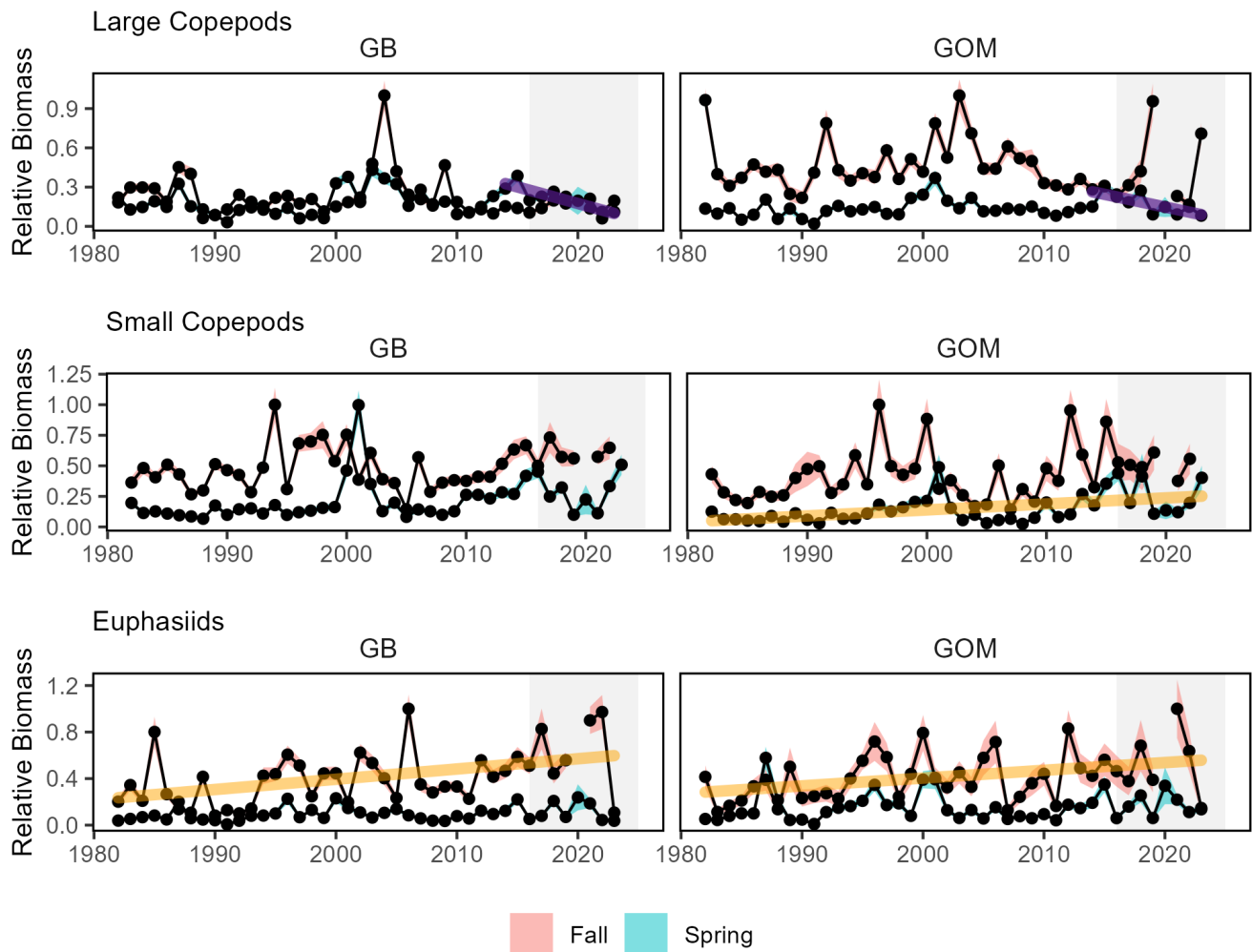
Figure 60: Changes in the abundance anomalies of three zooplankton groups in Georges Bank (GB, left) and the Gulf of Maine (GOM, right): large copepods (includes ( Calanus finmarchicus , top), small copepods (including ( C. typicus and ( Pseudocalanus spp. ), and Euphausiids (bottom), with significant decreases (short-term, dark purple) in large copepods and long-term increases (orange) in GOM small copepods and GB and GOM euphausiids.
