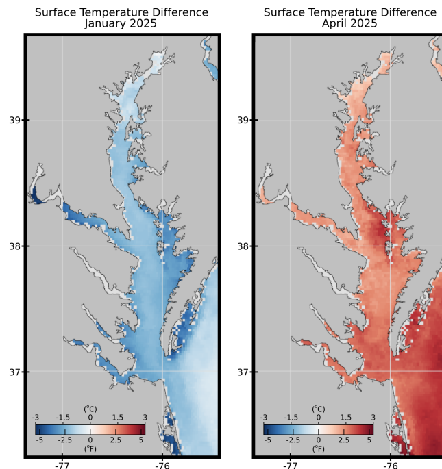
Figure 74: January 2025 (left) and April 2025 (right) sea surface temperature differences compared to the respective monthly climatological means. Sea Surface Temperature (SST) is from the NOAA Advanced Clear-Sky Processor for Ocean (ACSPO) Super-collated SST (climatology range 2000-2020).
