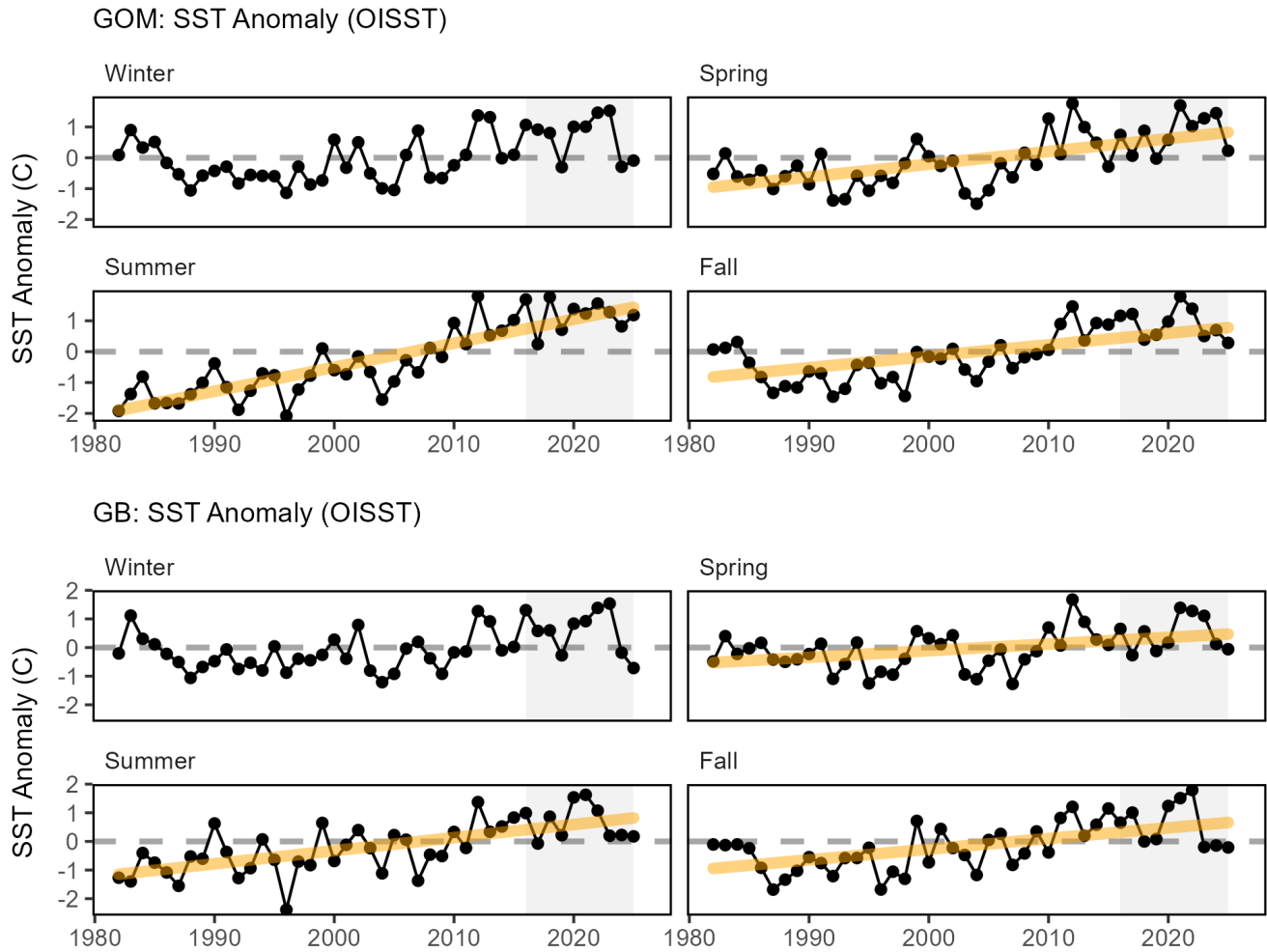
Figure 43: Seasonal Optimum Interpolation Sea Surface Temperature (OISST) anomaly by season for the Gulf of Maine (GOM, top) and Georges Bank (GB, bottom), with long-term increasing trends (orange).
