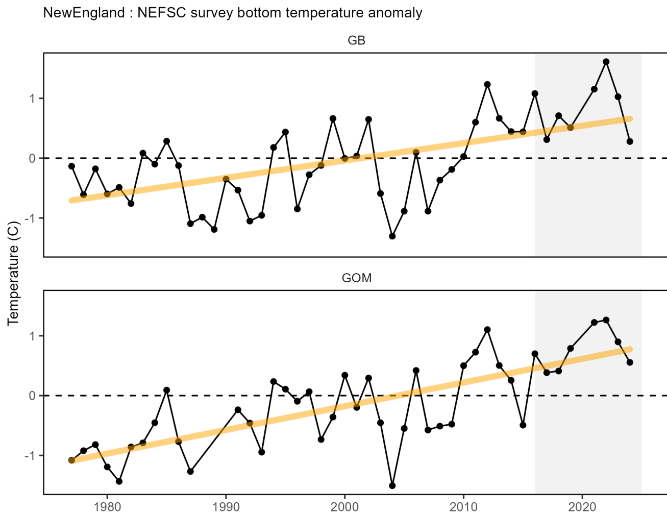
Figure 44: Annual in situ bottom temperature anomaly for Georges Bank (top) and the Gulf of Maine (bottom), with long-term increasing trends (orange).
