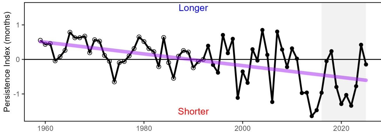
Figure 51: The Mid-Atlantic Bight Cold Pool persistence index based on bias-corrected Regional Ocean Modeling System-Northwest Atlantic(open circles) and GLORYS (closed circles), with significant long-term decline (purple).
