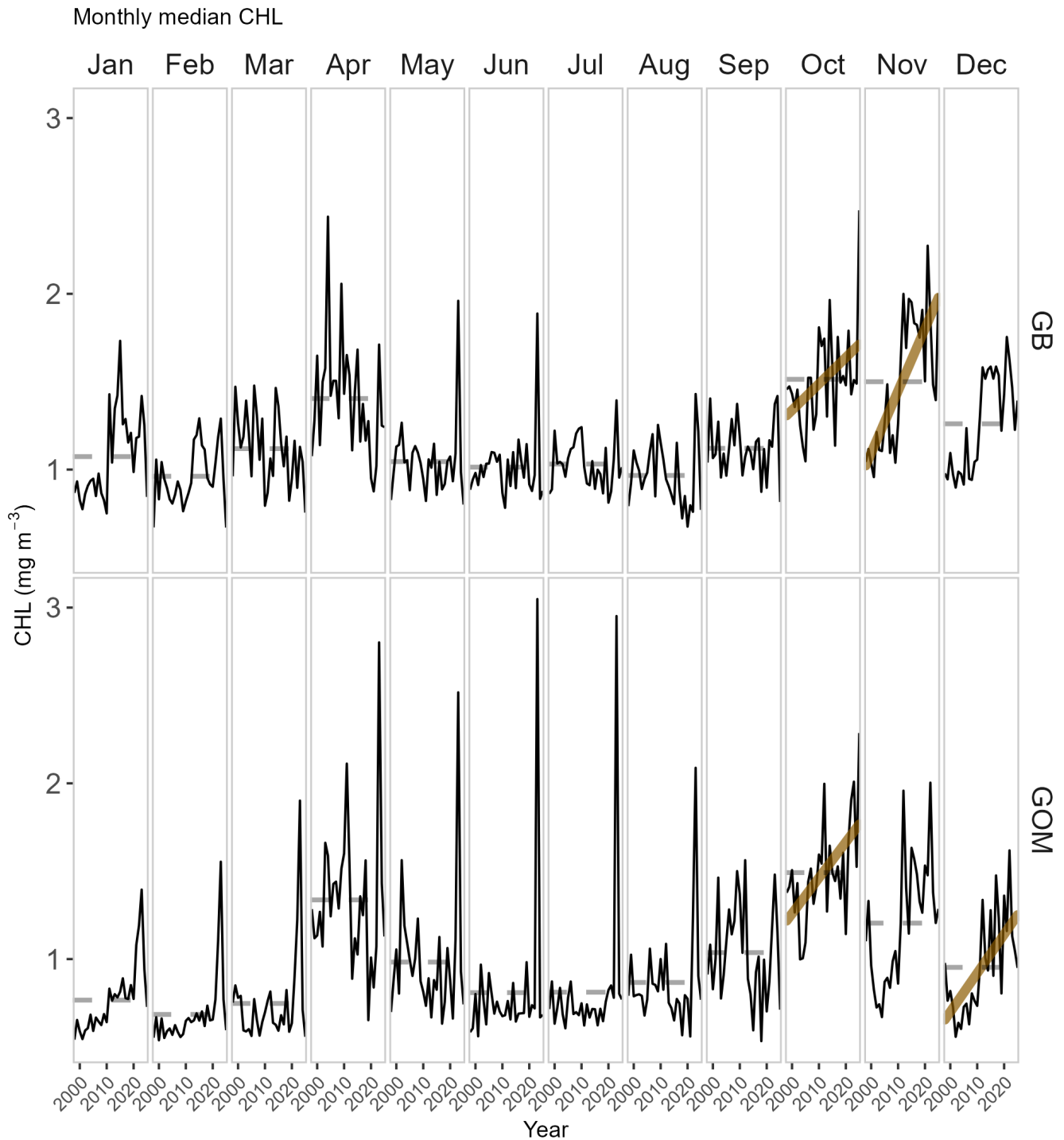
Figure 52: Monthly median chlorophyll a concentration time series for Georges Bank (top) and Gulf of Maine (bottom), with increasing long-term trends (orange).
