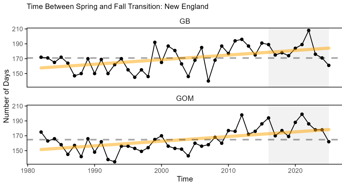
Figure 50: Ocean summer length in New England (Georges Bank, top; Gulf of Maine, bottom): the annual total number of days between the spring thermal transition date and the fall thermal transition date (black), with a long-term increasing trend (orange). Transition dates are based on sea surface temperatures.
