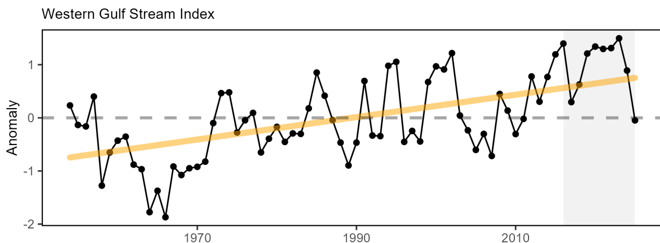
Figure 47: Index representing changes in the location of the western (between 64 and 55 degrees W) Gulf Stream north wall (black). Positive values represent a more northerly Gulf Stream position, with long-term increasing trend (orange).
