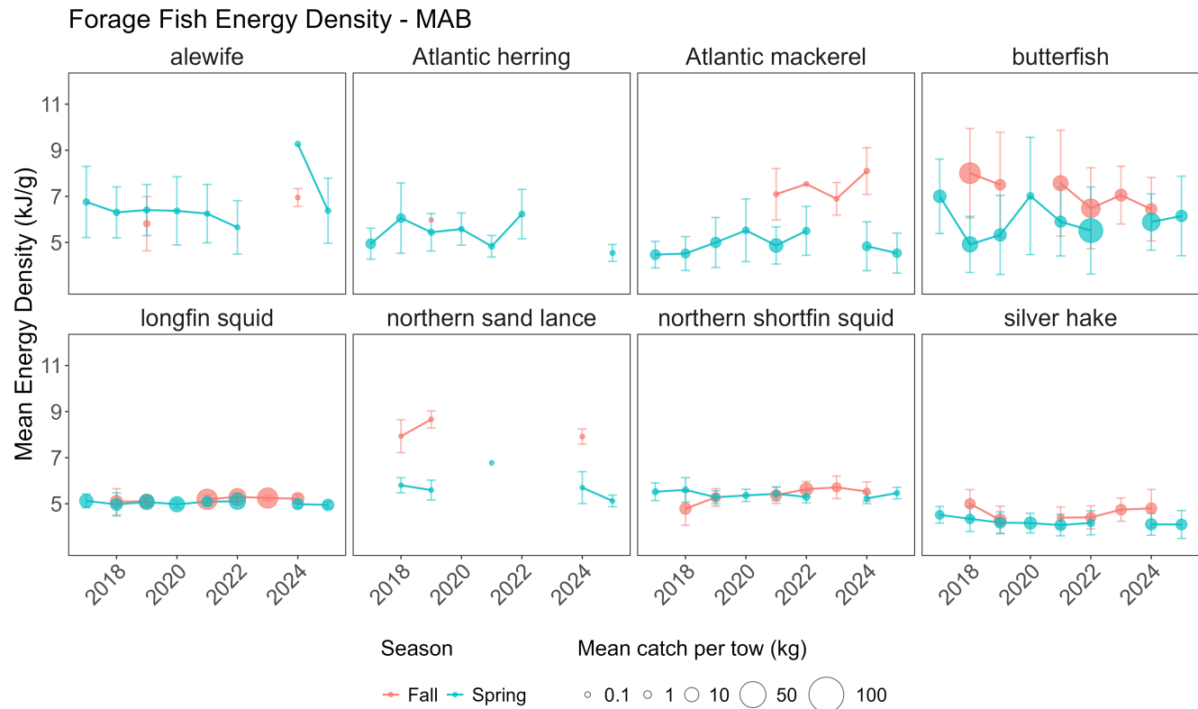
Figure 51: Energy density (mean and standard deviation) of eight forage species from NEFSC bottom trawl surveys by season and year for the MAB. Symbol size represents abundance (mean kg/tow) estimated from bottom trawl survey tows in the MAB.
