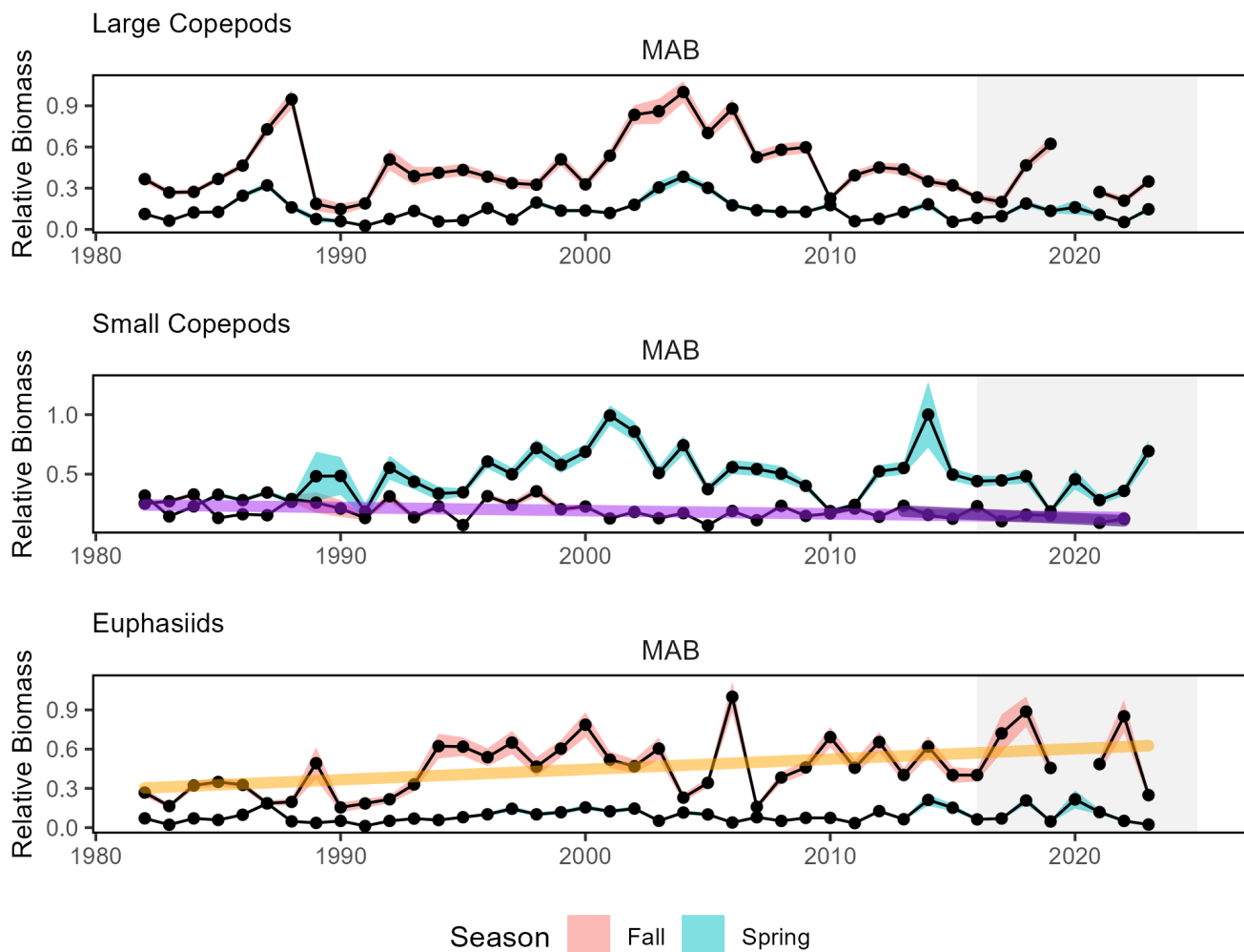
Figure 54: Changes in the abundance anomalies of three zooplankton groups in the [location]: large copepods (includes Calanus finmarchicus , top), small copepods (middle), and Euphausiids (bottom), with significant decreases (short-term, dark purple; long-term, light purple) in small copepods and long-term increases (orange) in Euphausiids.
