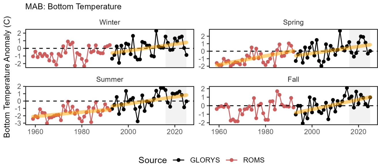
Figure 41: GLORYS (black) and debiased ROMS (red) seasonal bottom temperature anomaly in the MAB, with long-term increasing trends (orange).
