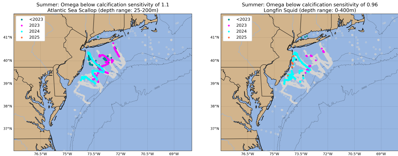
Figure 61: Locations where bottom aragonite saturation state ( \Omega_{Arag} ; summer only: June-August) were at or below the laboratory-derived sensitivity level for Atlantic sea scallop (left panel) and longfin squid (right panel) for the time periods 2007-2022 (dark cyan), 2023 only (magenta) and 2024 only (cyan). Gray circles indicate locations where bottom \Omega_{Arag} values were above the species specific sensitivity values.
