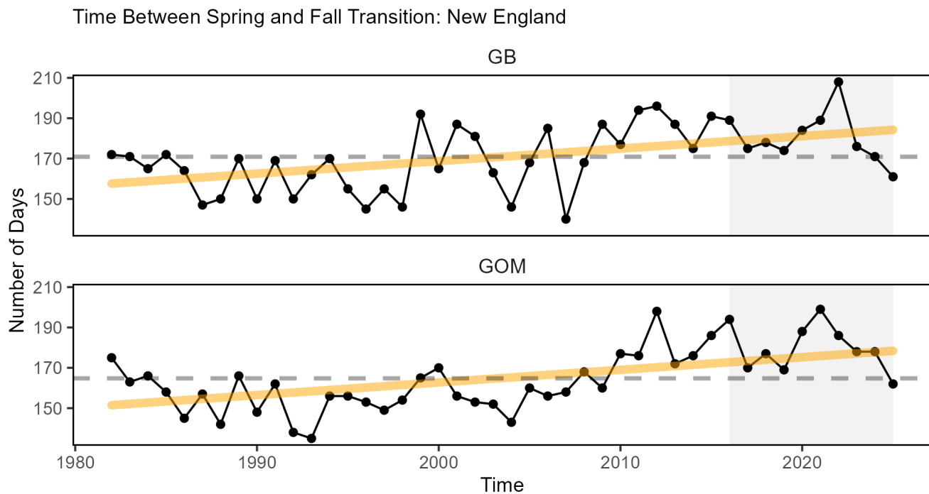
Figure 46: Ocean summer length in New England (Georges Bank, top; Gulf of Maine, bottom): the annual total number of days between the spring thermal transition date and the fall thermal transition date (black), with a long-term increasing trend (orange). Transition dates are based on sea surface temperatures.
