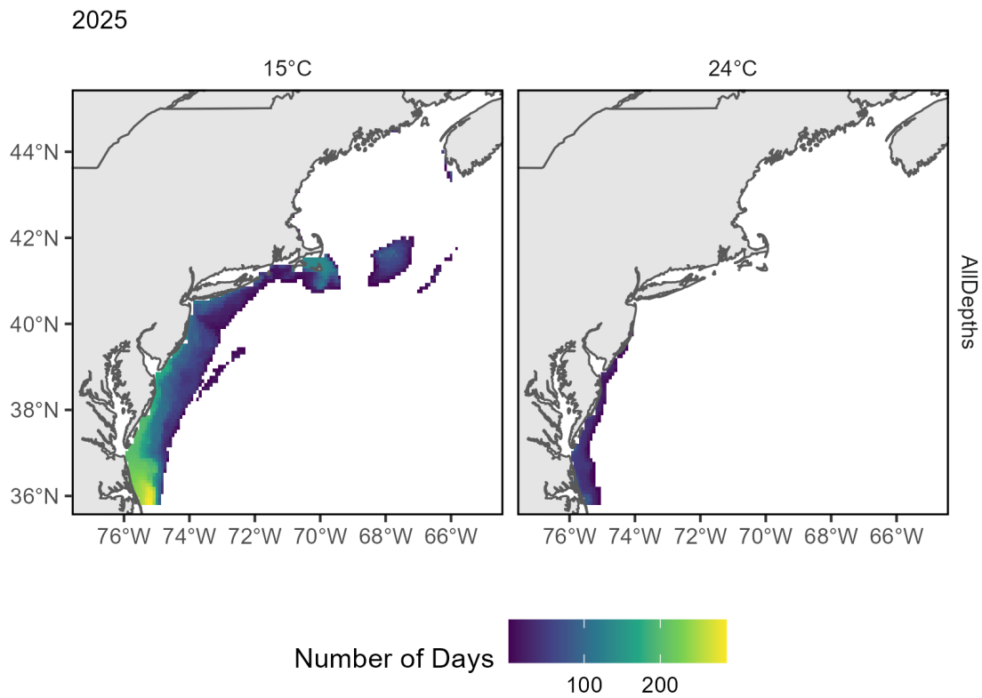
Figure 59: The number of days in 2025 where bottom temperature exceeds 15 degrees (left) and 24 degrees (right) based on the GLORYS 1/12 degree grid.
