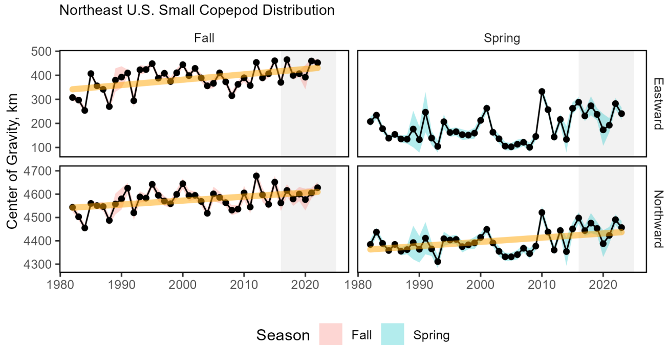
Figure 38: Eastward (top) and northward (bottom) shifts in the center of gravity for small copepod species on the Northeast U.S. Shelf in fall (left) and spring (right).
