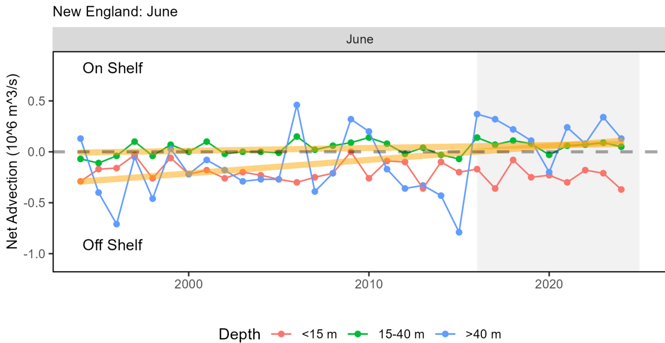
Figure 60: Net advection in June across the Southern New England and Georges Bank continental shelf break within 3 depth bands, with increasing long-term trends in the middle and bottom depths (orange).
