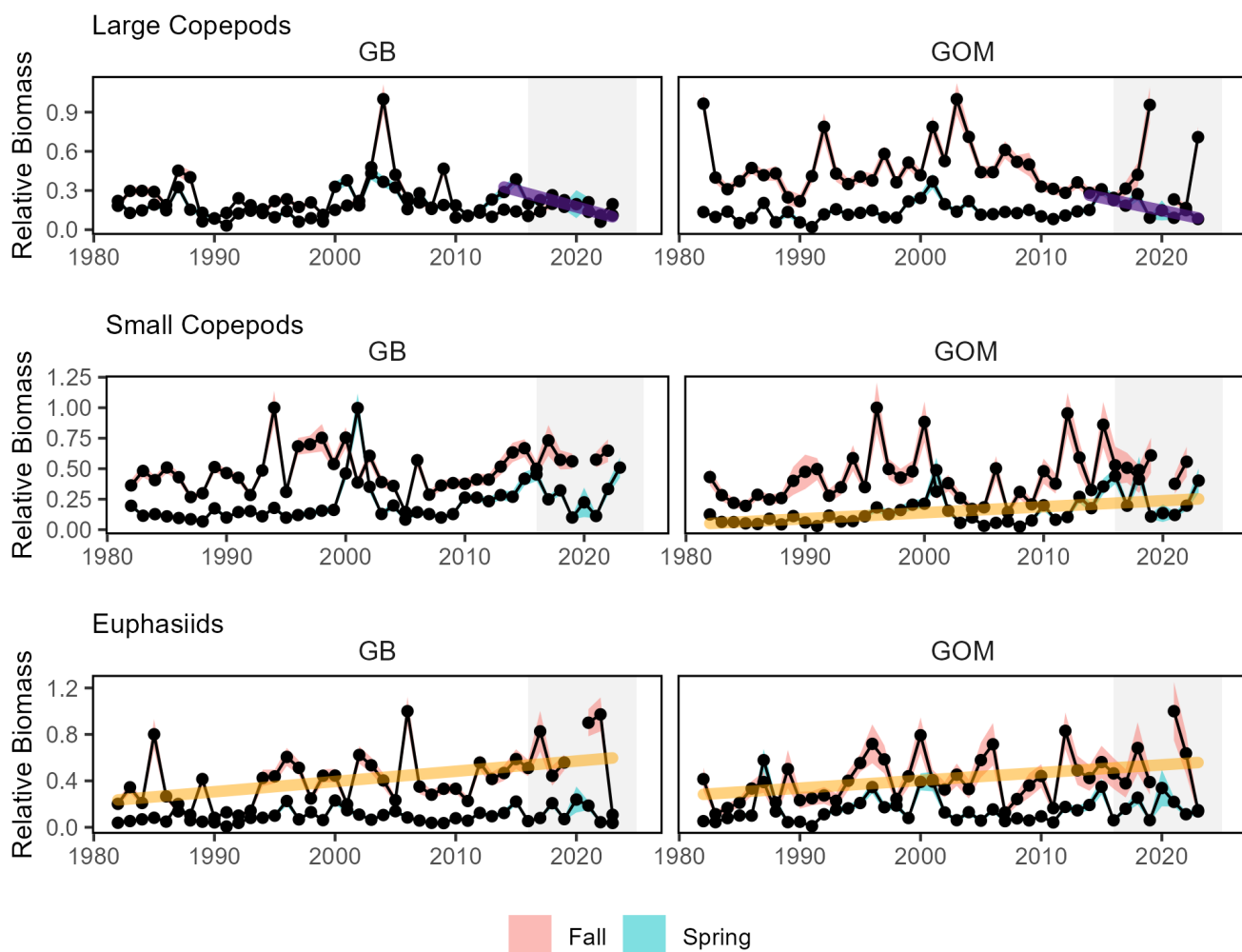
Figure 56: Changes in the abundance anomalies of three zooplankton groups in the [location]: large copepods (includes Calanus finmarchicus , top), small copepods (middle), and Euphausiids (bottom), with significant decreases (short-term, dark purple) in large copepods and long-term increases (orange) in GOM small copepods and GB and GOM euphausiids.
