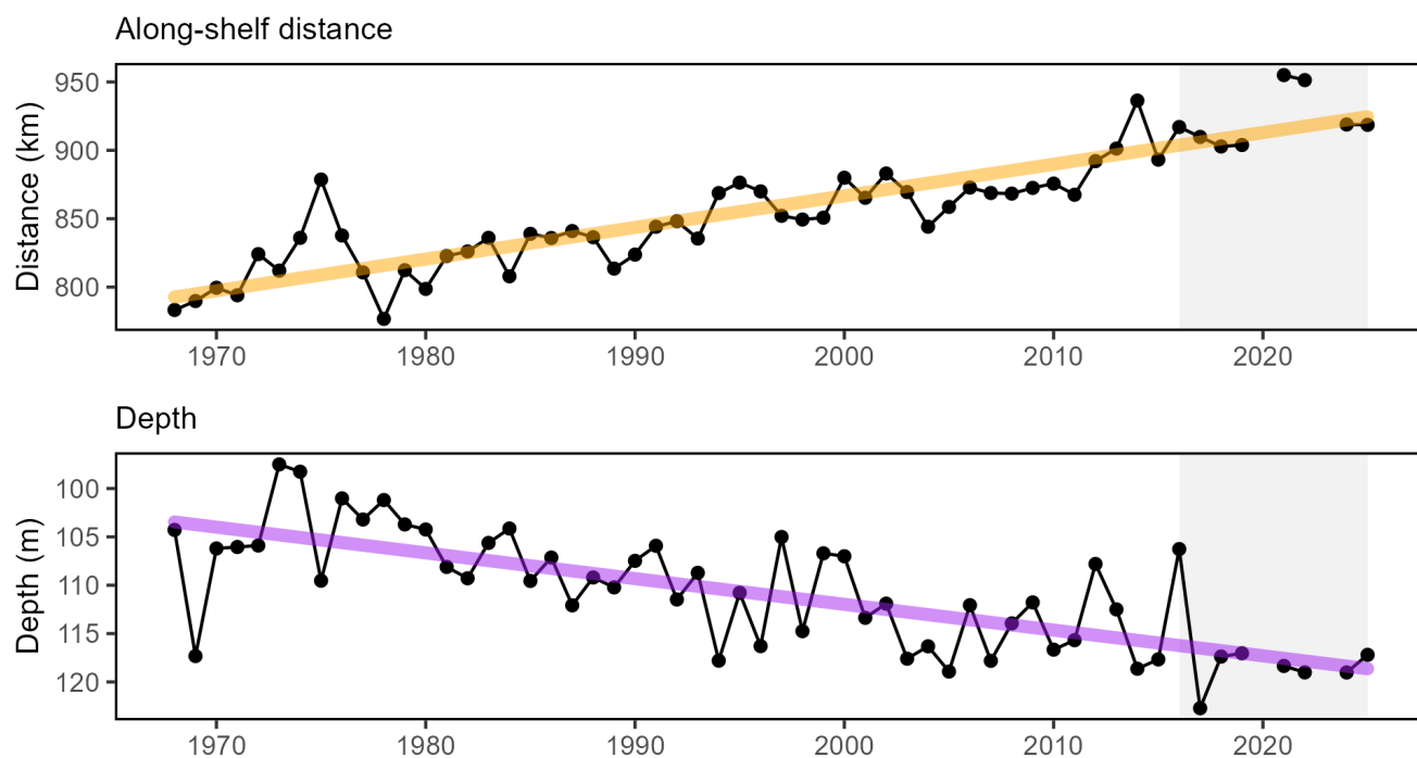
Figure 31: Aggregate species distribution metrics for species in the Northeast Large Marine Ecosystem: along shelf distance with long-term increasing trend (orange), and depth with long-term decreasing trend indicating deeper water (purple).
