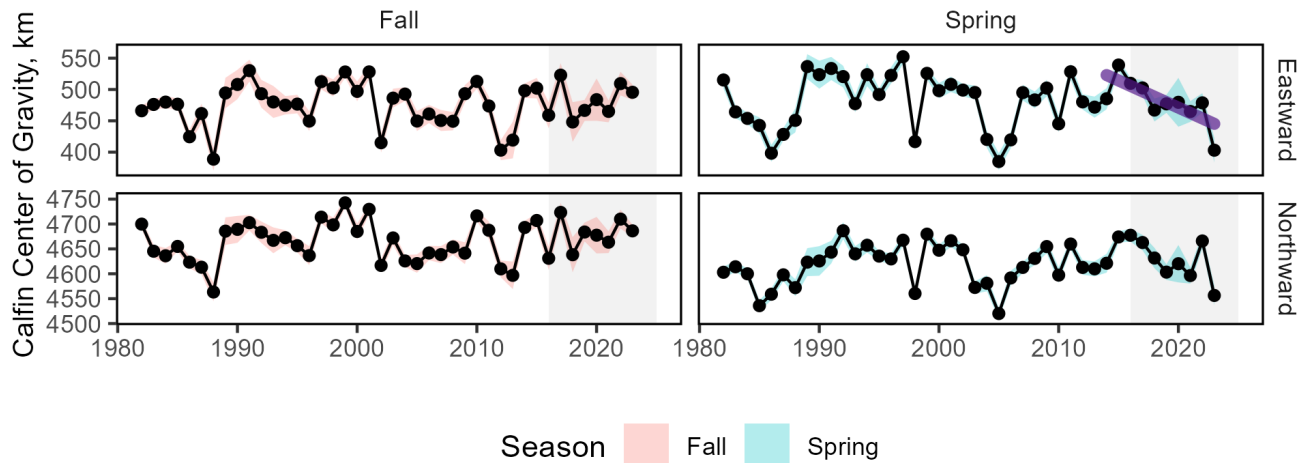
Figure 33: Eastward (top) and northward (bottom) shifts in the center of gravity for ( Calanus finmarchicus ) on the Northeast U.S. Shelf in fall (left) and spring (right)
