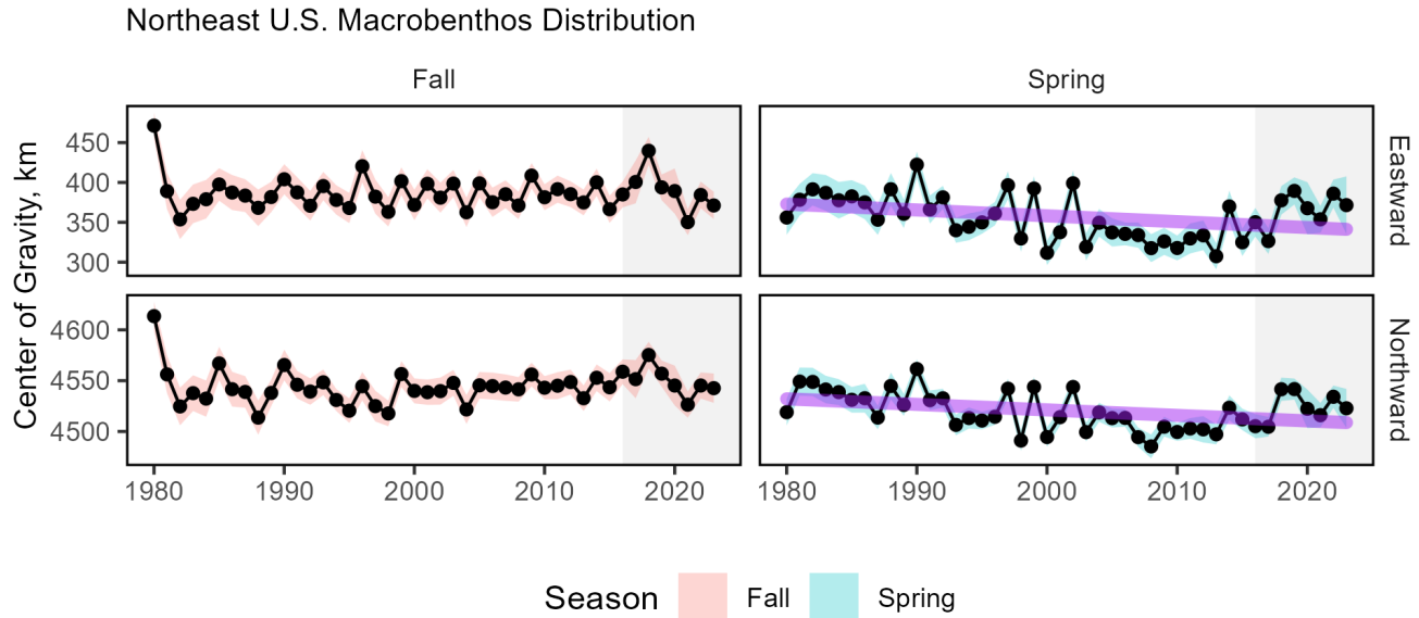
Figure 36: Eastward (top) and northward (bottom) shifts in the center of gravity for macrobenthos species on the Northeast U.S. Shelf in fall (left) and spring (right), with decreasing trends (purple) for spring eastward and northward center of gravity.
