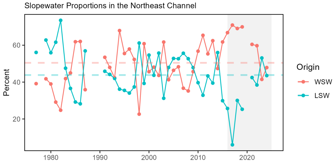
Figure 64: The proportion of Warm Slope Water (WSW) and Labrador Slope Water (LSW) entering the Gulf of Maine through the Northeast Channel from 1977 to 2024. The red and teal dashed lines represent the long-term proportion averages for the WSW and LSW respectively.
