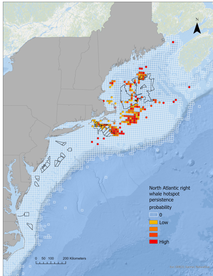
Figure 62: North Atlantic Right Whale persistent hotspots (red shading) and Wind Energy Areas (black outlines).
