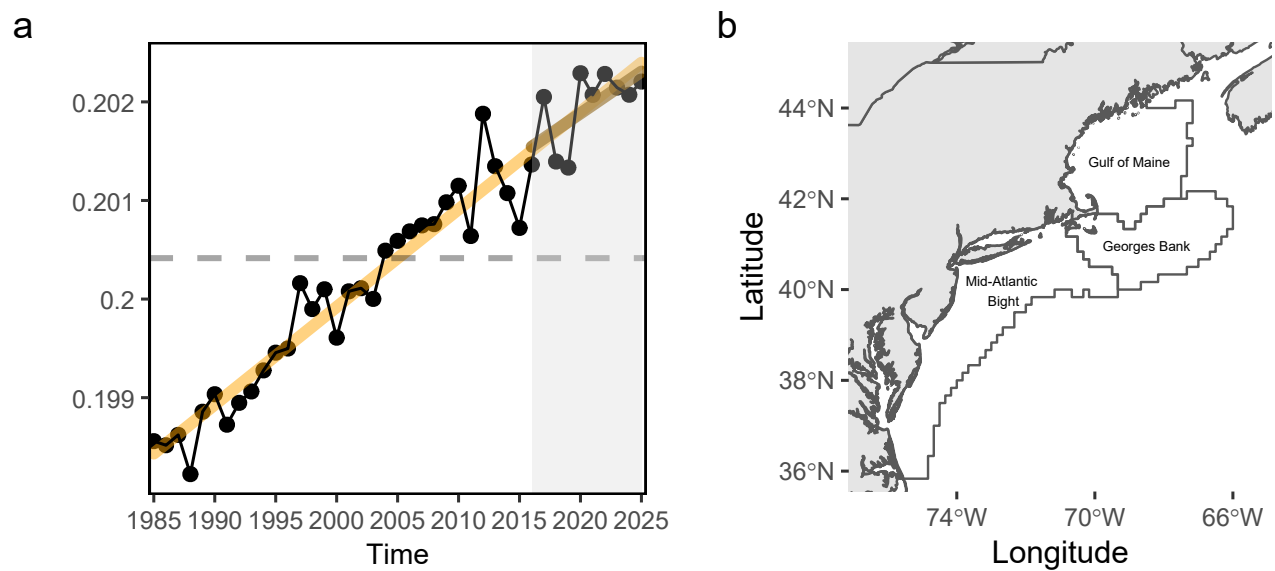
Figure 67: Document orientation. a) Key to figures: orange line - significant long-term increasing trend (purple for decreasing), dark orange line - significant increasing short-term trend (dark purple for decreasing), dashed line - time-series mean. b) The Northeast Large Marine Ecosystem: Ecological production units (EPUs) defined for the Gulf of Maine (GOM), Georges Bank (GB), and the Mid-Atlantic Bight (MAB).
