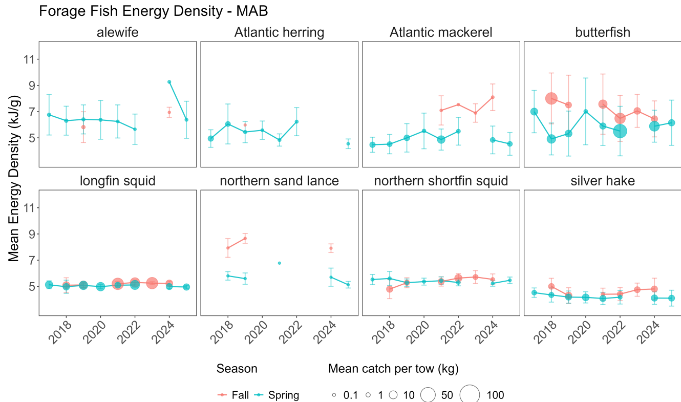
Figure 50: Energy density (mean and standard deviation) of eight forage species from NEFSC bottom trawl surveys by season and year for the MAB. Symbol size represents abundance (mean kg/tow) estimated from bottom trawl survey tows in the MAB.
