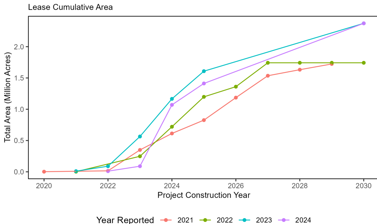
Figure 61: Total area proposed for wind development on the Northeast Shelf through 2030.
