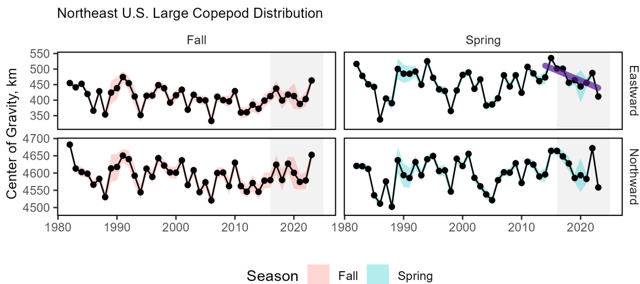
Figure 40: Eastward (top) and northward (bottom) shifts in the center of gravity for large copepod species ( Calanus finmarchicus , Metridia lucens , Calanus minor , Eucalanus sp., Calanus spp.) on the Northeast U.S. Shelf in fall (left) and spring (right).
