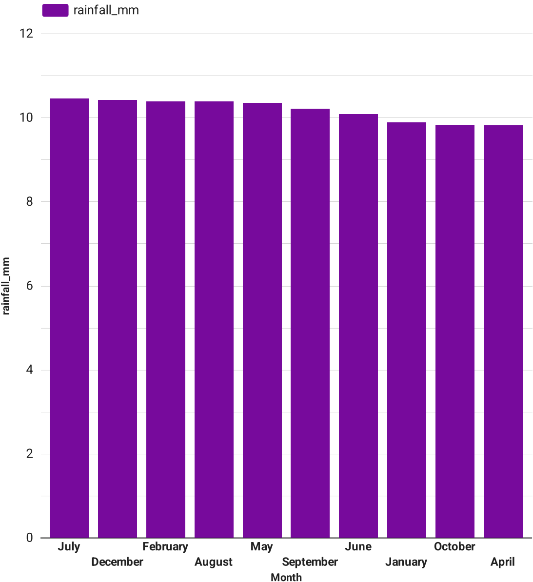
Month Rain-Fall Average
