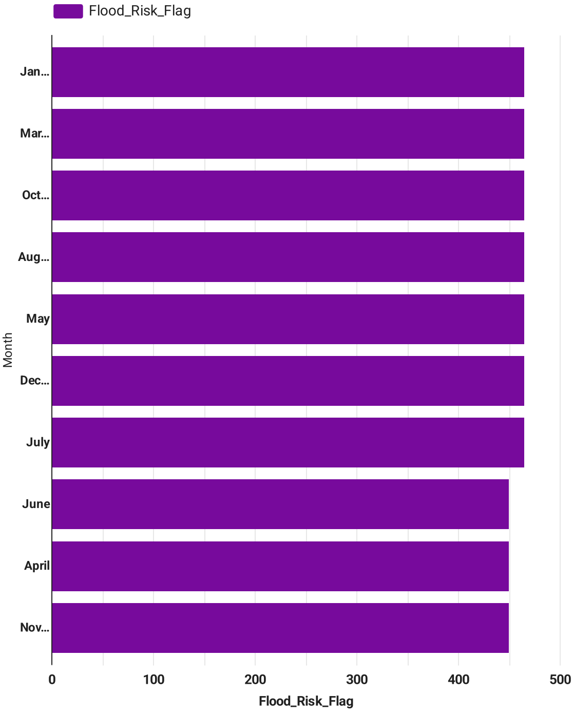
Count Of Flood_Risk_Flag by Month
