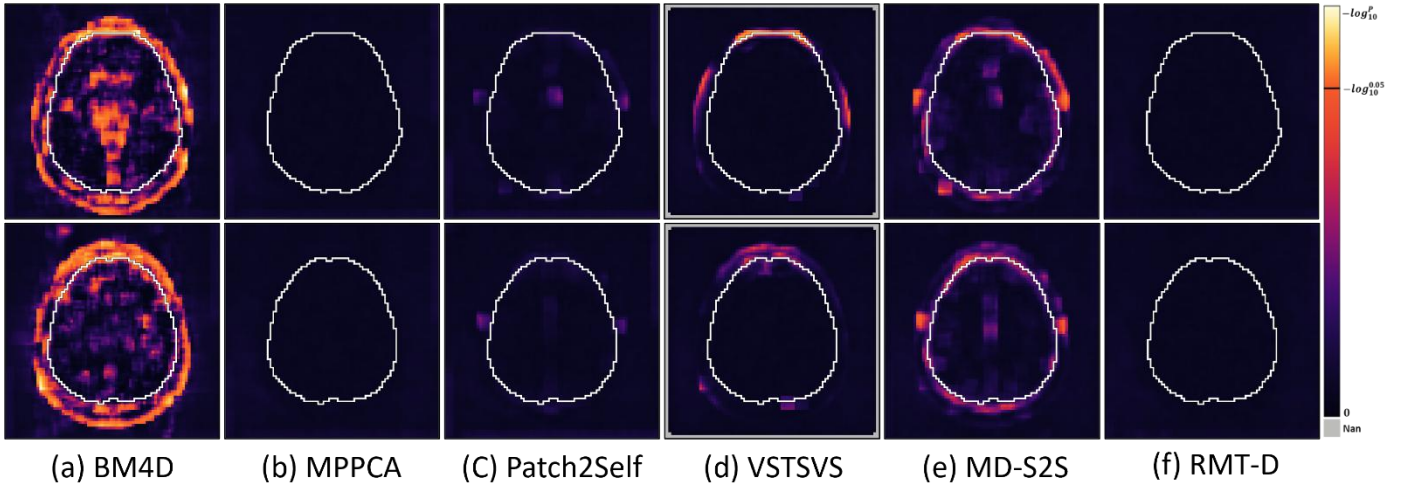
Heatmaps of local K-S diagnostics for residual Gaussianity in acquired human rs-fMRI data. The two rows correspond to slices 16 and 23, respectively. The residuals were standardized using the RMT-D noise-scale estimate as a common normalization reference. Each voxel displays -\log_{10}[\text{mean}_t\{p_{KS}(v, t)\}] , and the reference threshold is -\log_{10}(0.05) . Values above this threshold correspond to a temporally averaged p value below 0.05, whereas the remaining values indicate insufficient evidence to reject Gaussianity under this descriptive summary. The displayed values are not additionally truncated. Gray regions in the VSTSVS results denote boundary locations that were not processed because of the preset kernel size and therefore contain NaN values.
