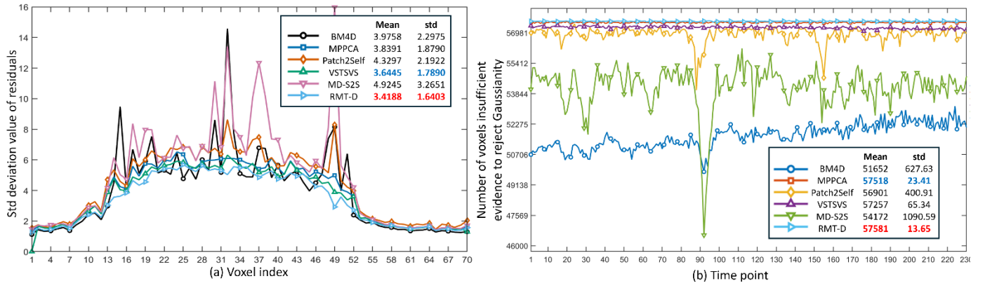
Residual statistics for acquired human rs-fMRI data. (a) Profiles extracted along the three-dimensional spatial diagonal from voxel (1,1,1) to (H, W, Z) from Fig.4(g)-(l). The horizontal axis denotes the voxel index along the path, and the vertical axis denotes the residual temporal standard deviation. Mean and standard deviation in the legend denote the mean and standard deviation of the profile values at the common valid path locations, respectively. (b) Number of foreground voxels at each time point for which there was insufficient evidence to reject Gaussianity. The horizontal axis denotes the time point, and the vertical axis denotes the number of voxels satisfying p_{KS} \geq 0.05 . Mean and standard deviation in the legend denote the temporal mean and standard deviation of the voxel-count trajectory, respectively.
