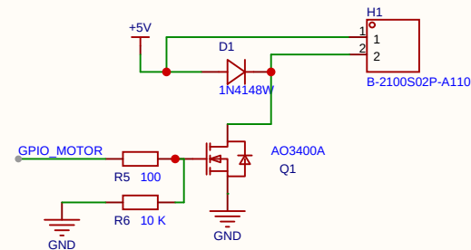
Vibration Driver
