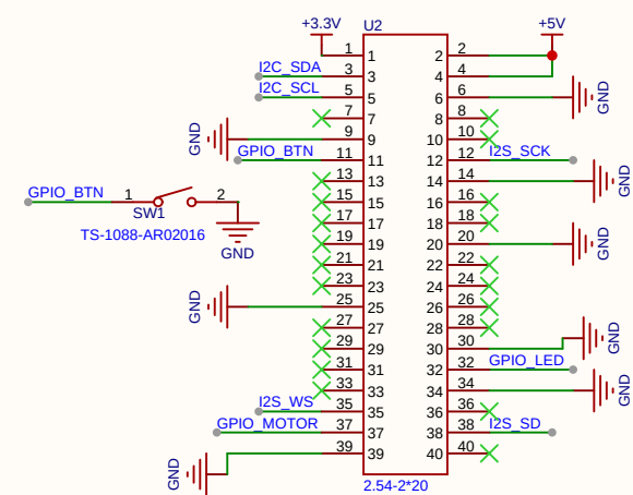
SBC 40-pin
