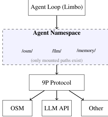
Figure 3: Namespace-bounded agent architecture. The agent sees only its mounted namespace; unmounted services do not exist. File operations replace JSON-RPC.
