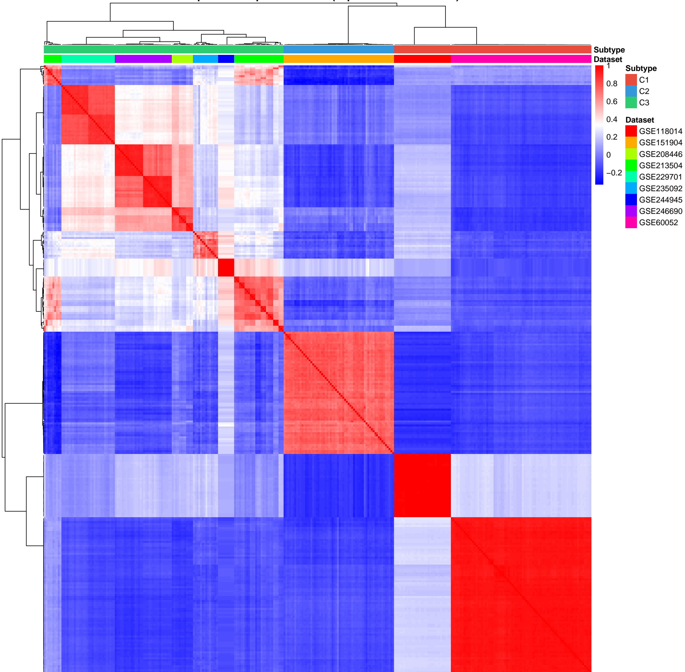
Sample-to-Sample Correlation (Top 1000 Variable Genes)
