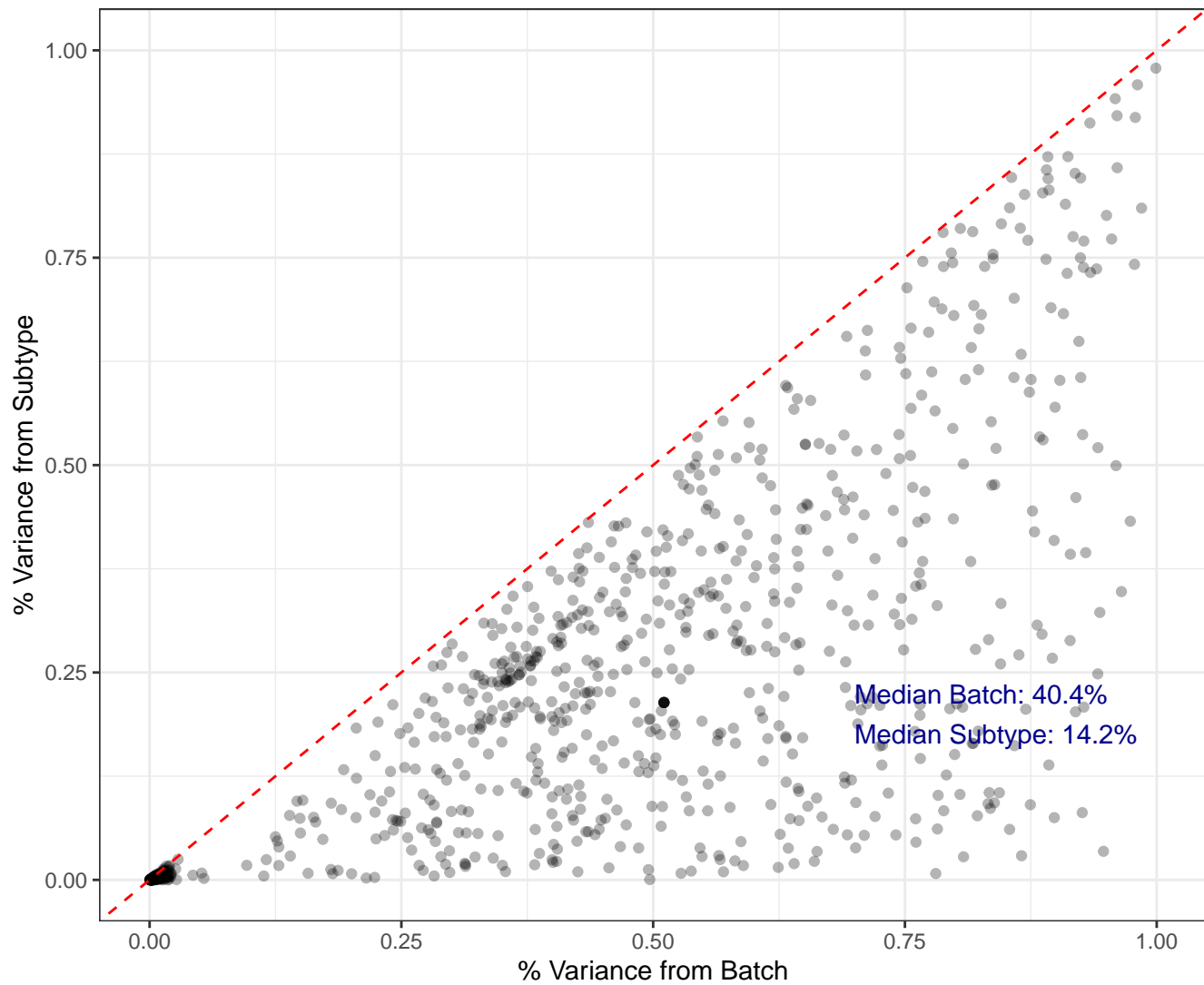
Variance Partitioning (1000 Random Genes)
