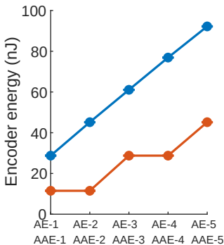
Encoder/decoder energy and MAE vs hidden layers
