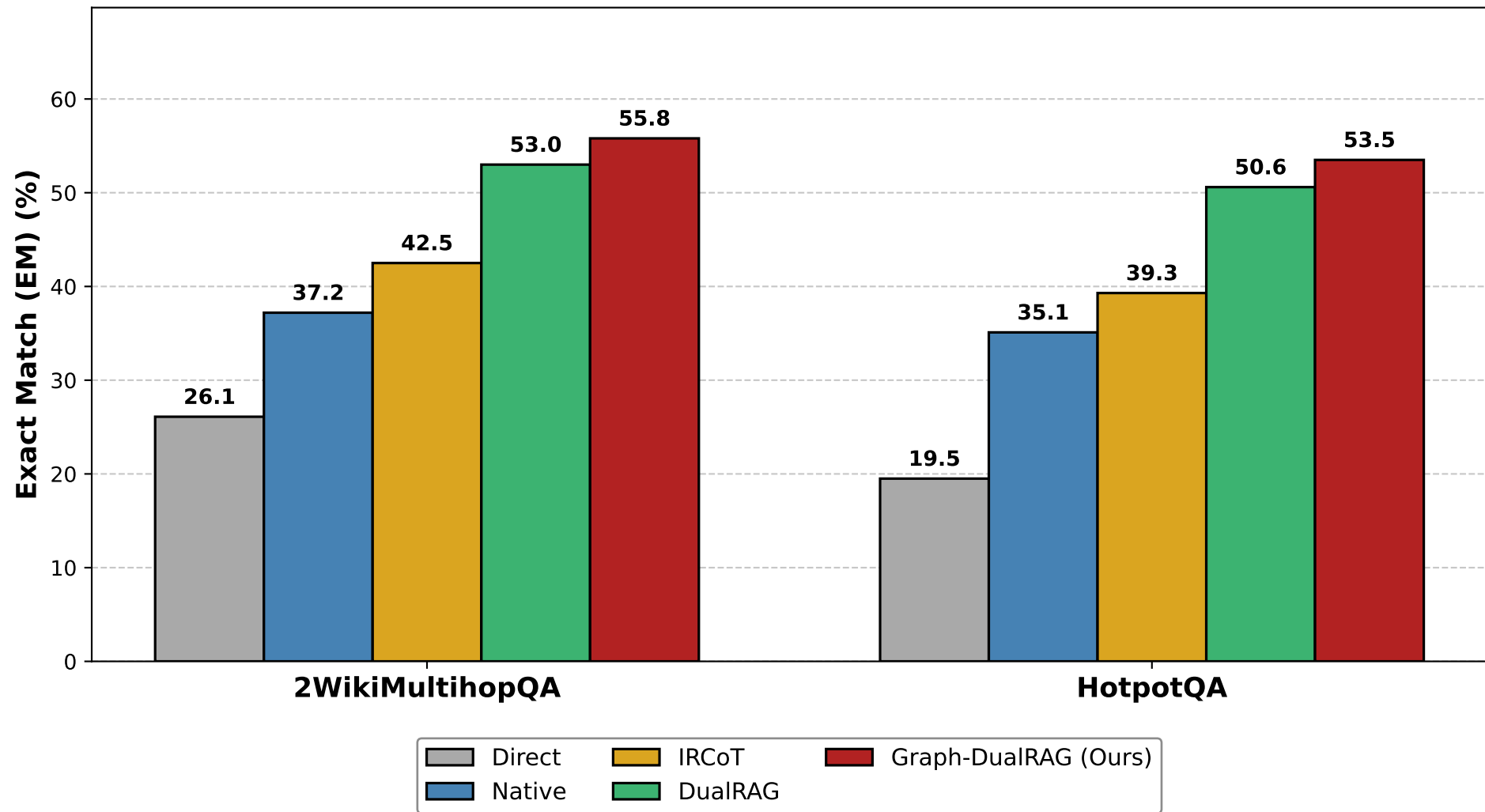
End-to-End Exact Match across Baselines
