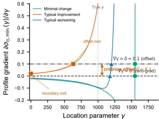
(a) \delta shifts the gradient criterion (per-sample effect varies)
