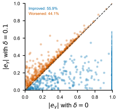
(c) Paired sample-level effect
