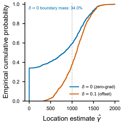
(b) Population shift in \hat{\gamma}
