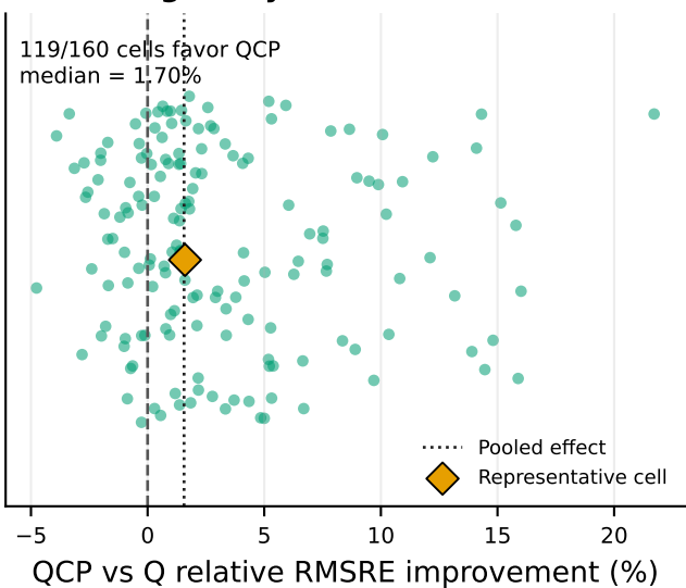
C What QCP changes relative to Q
