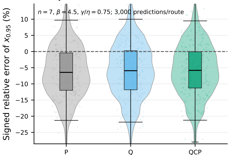
B Representative fixed-truth cell
