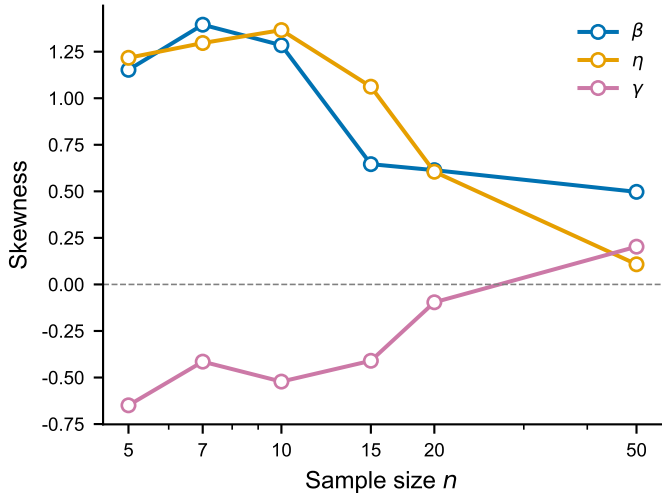
(a) Skewness
