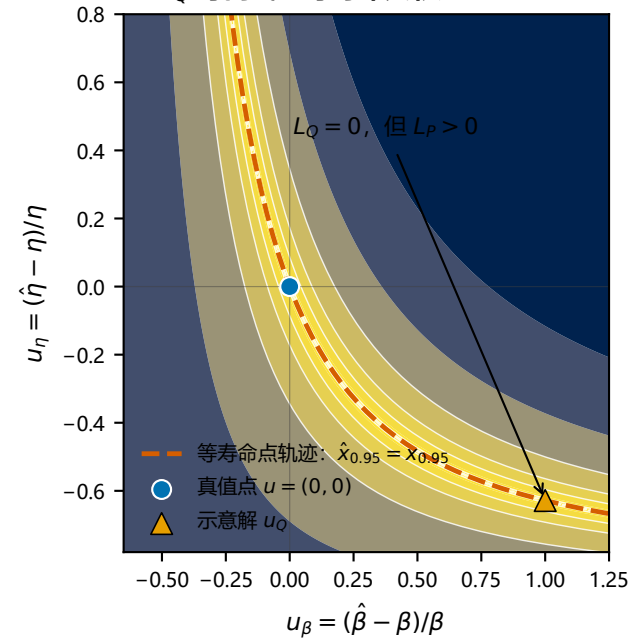
A L_Q 等高线与等寿命点轨迹
