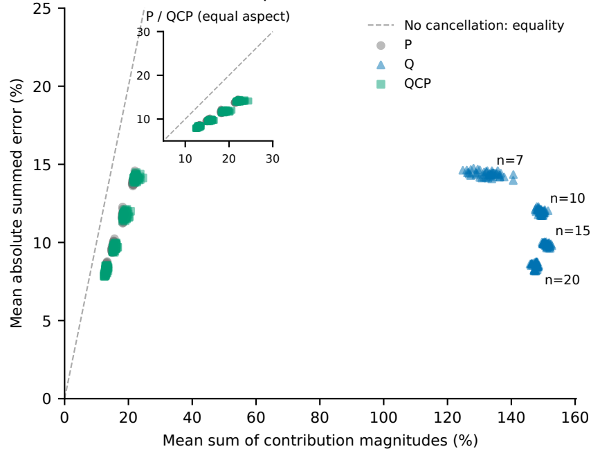
D Within-prediction cancellation
