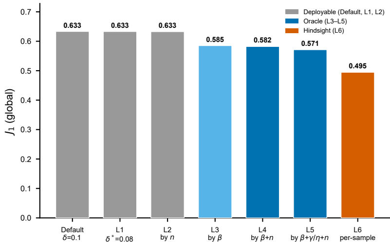
(a) Accuracy ladder: Default \rightarrow L6
