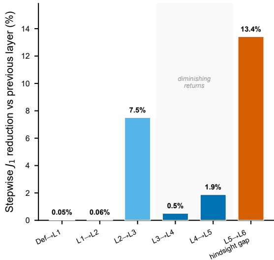
(b) Stepwise information gains and hindsight gap
