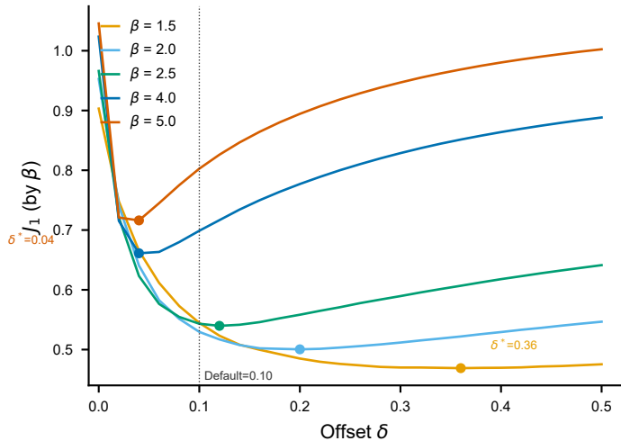
(b) \delta -risk by shape parameter \beta
