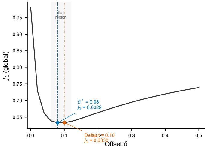
(a) Global \delta -risk curve
