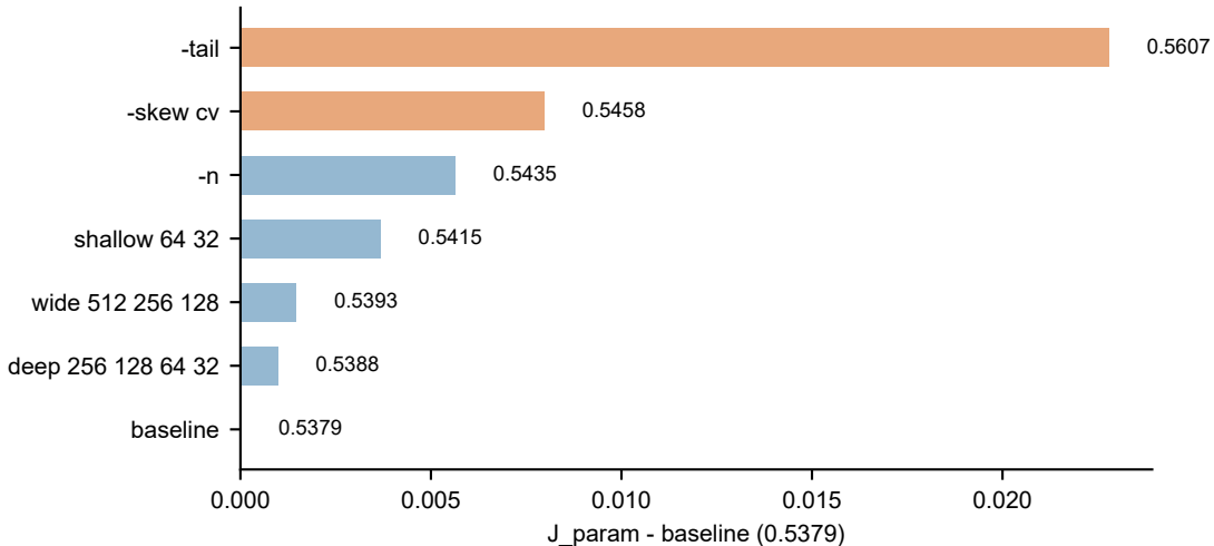
Ablation: J_param by Feature/Architecture
