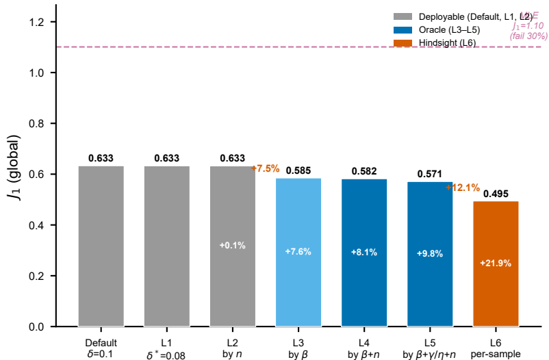
(a) Accuracy ladder: Default \rightarrow L6
