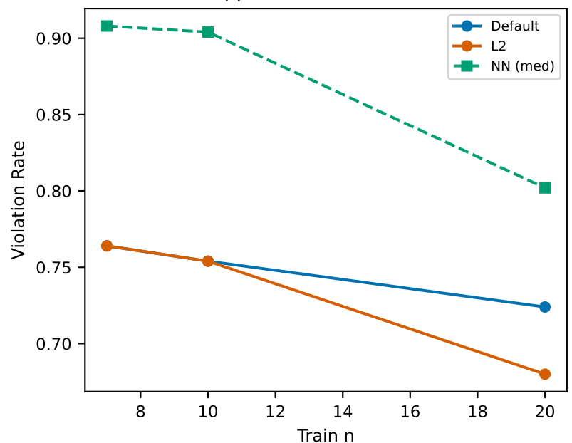
Support-Set Violation Rate
