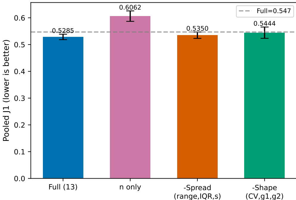
E4a: Feature Group Ablation
