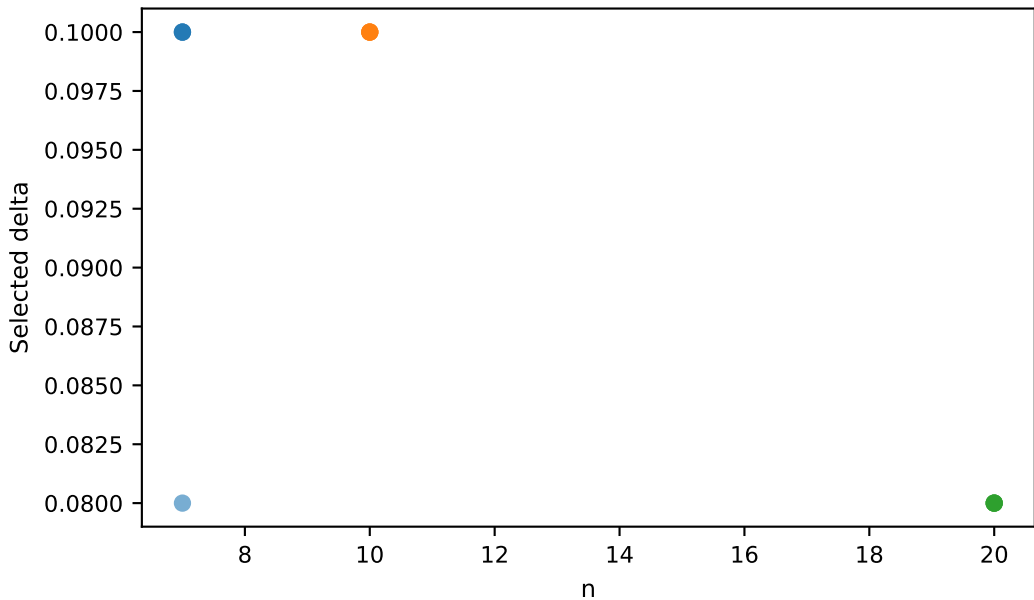
S1: L2 Cross-Fit Selected Delta by Fold and n
