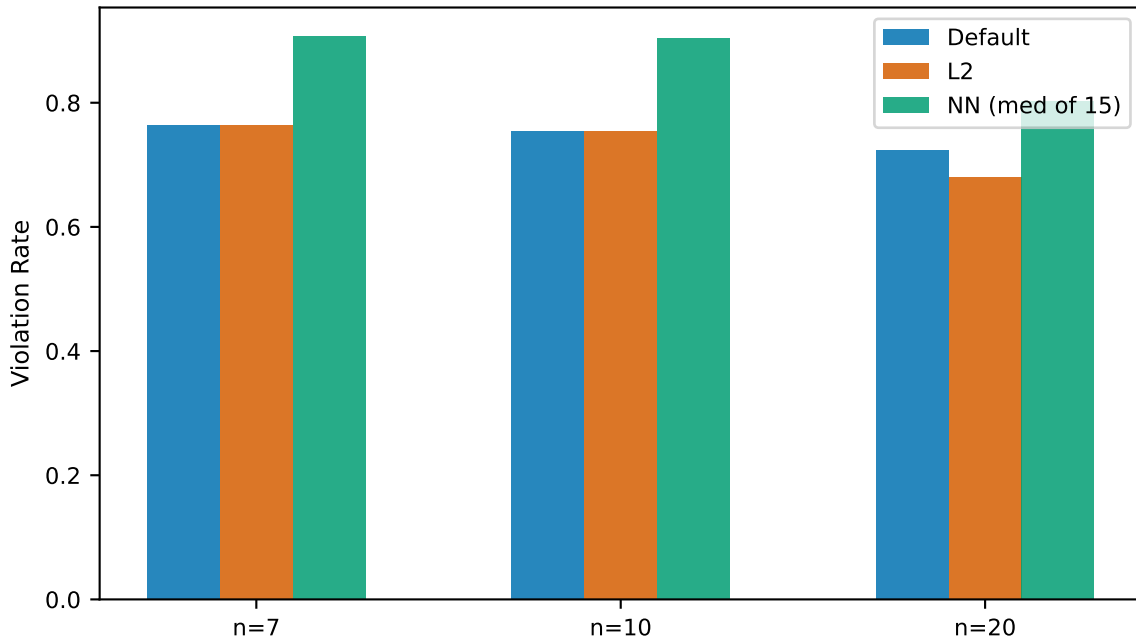
S8: Support-Set Violation by Method
