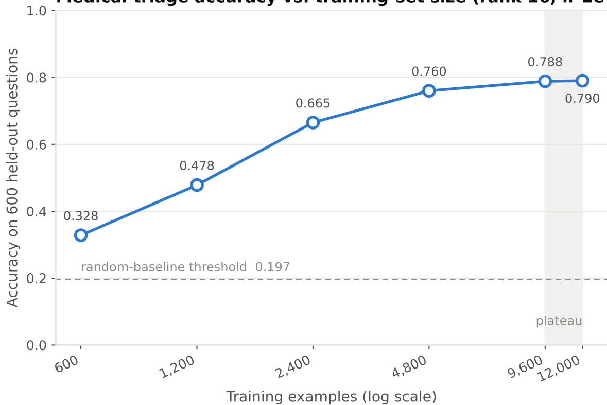
Medical triage accuracy vs. training-set size (rank 16, lr 2e-4)
