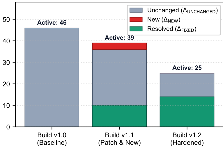
Vulnerability Count
