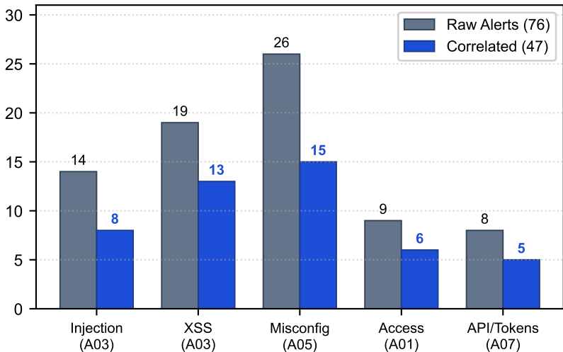
Finding Count
