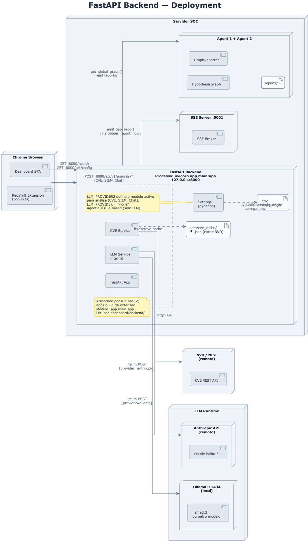
Figure 4: Diagrama de Deployment
