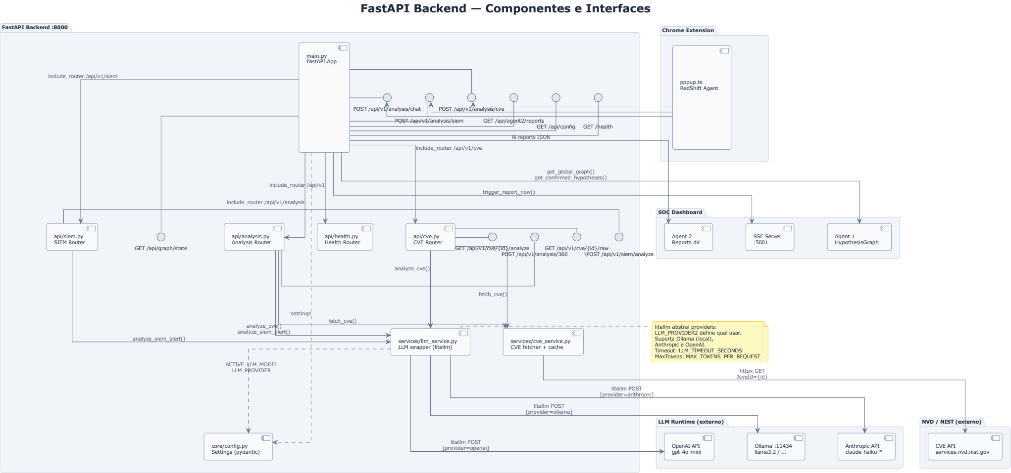
Figure 3: Componentes e Interfaces
