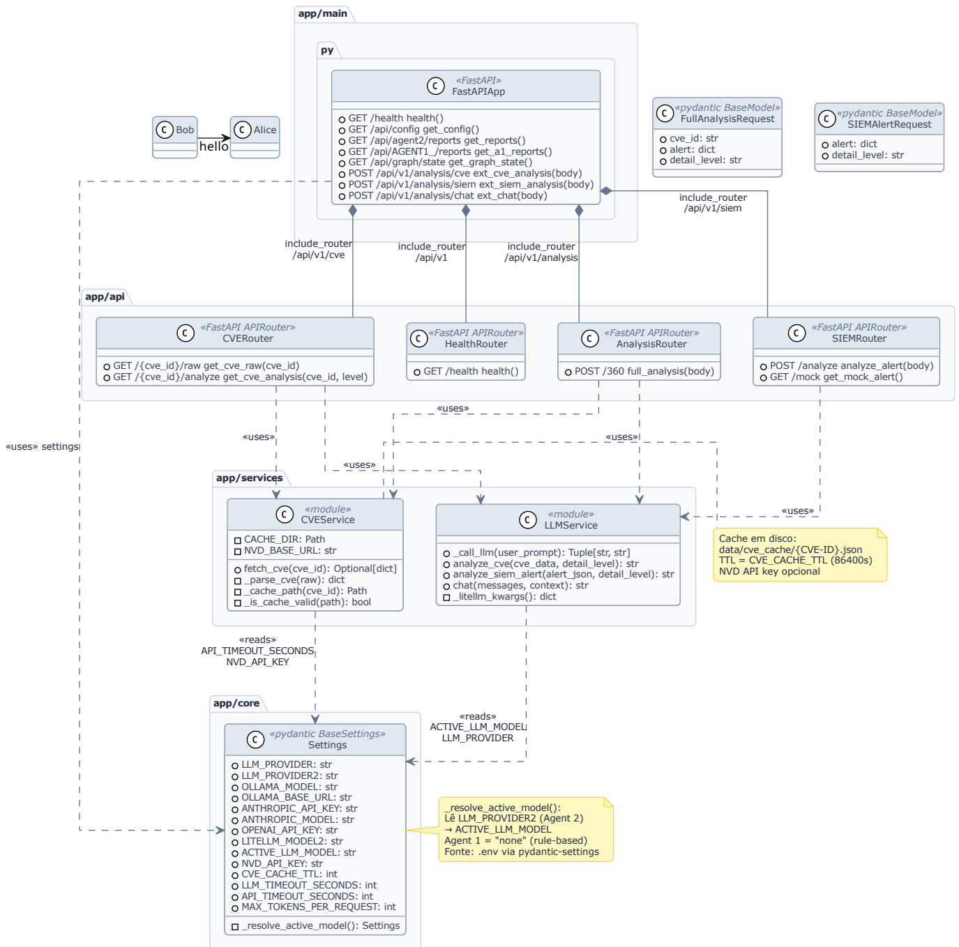
Figure 2: Diagrama de Classes
