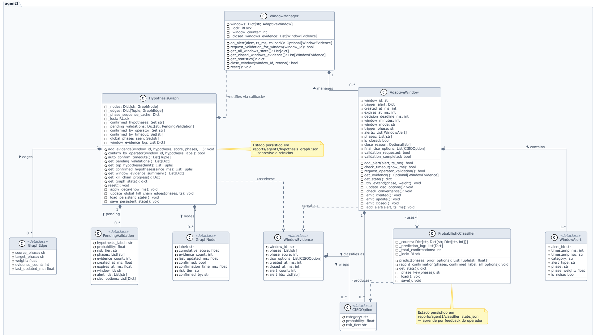
Figure 3: Diagrama de Classes
