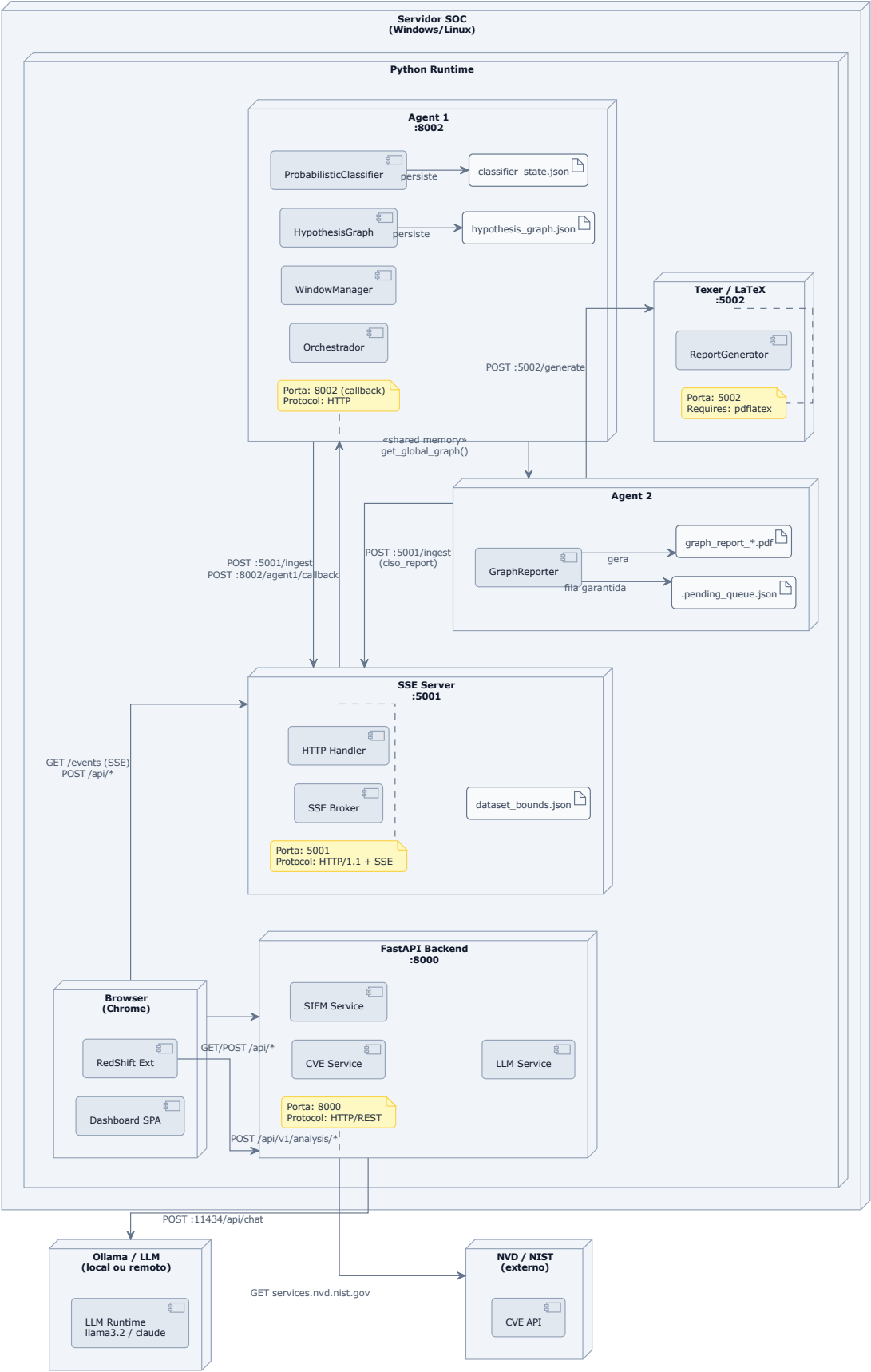
Figure 5: Diagrama de Deployment
