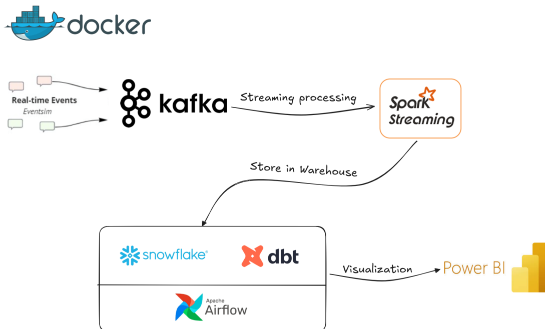
Figure 4.1: Streamify end-to-end architecture: from event simulation to BI dashboard.
