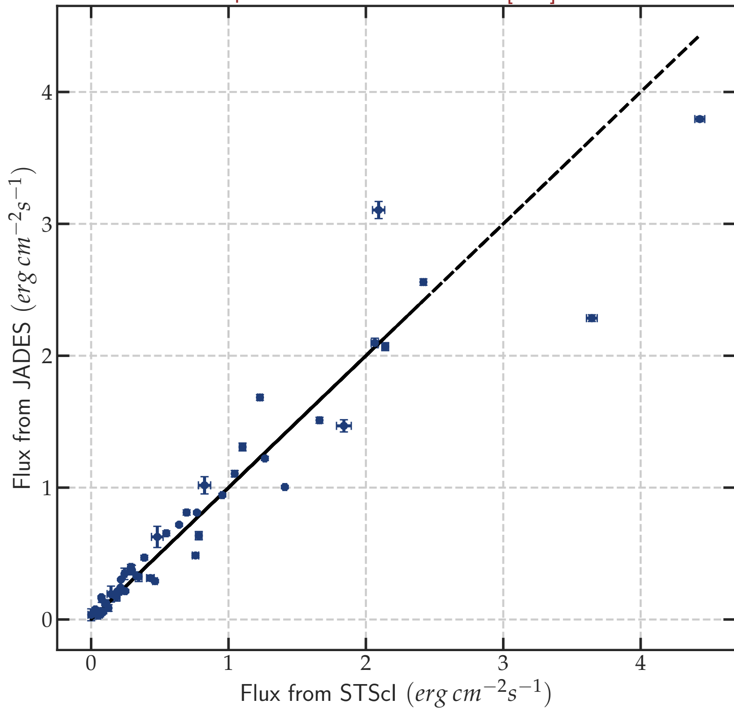
Comparison of flux estimates for [OIII]5007
