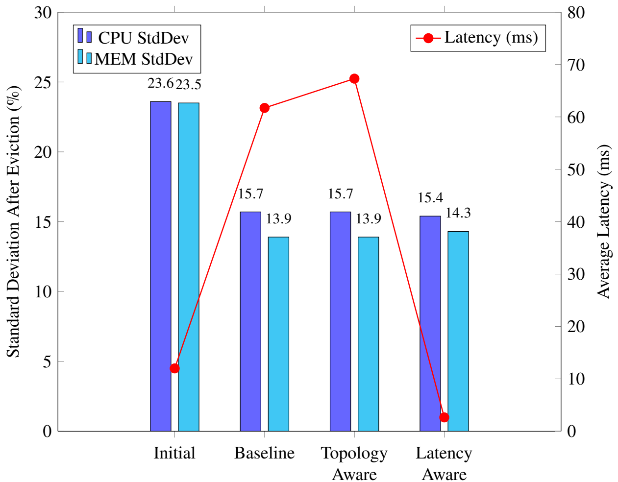
Figure 19. Cluster Balance vs. Network Performance.
