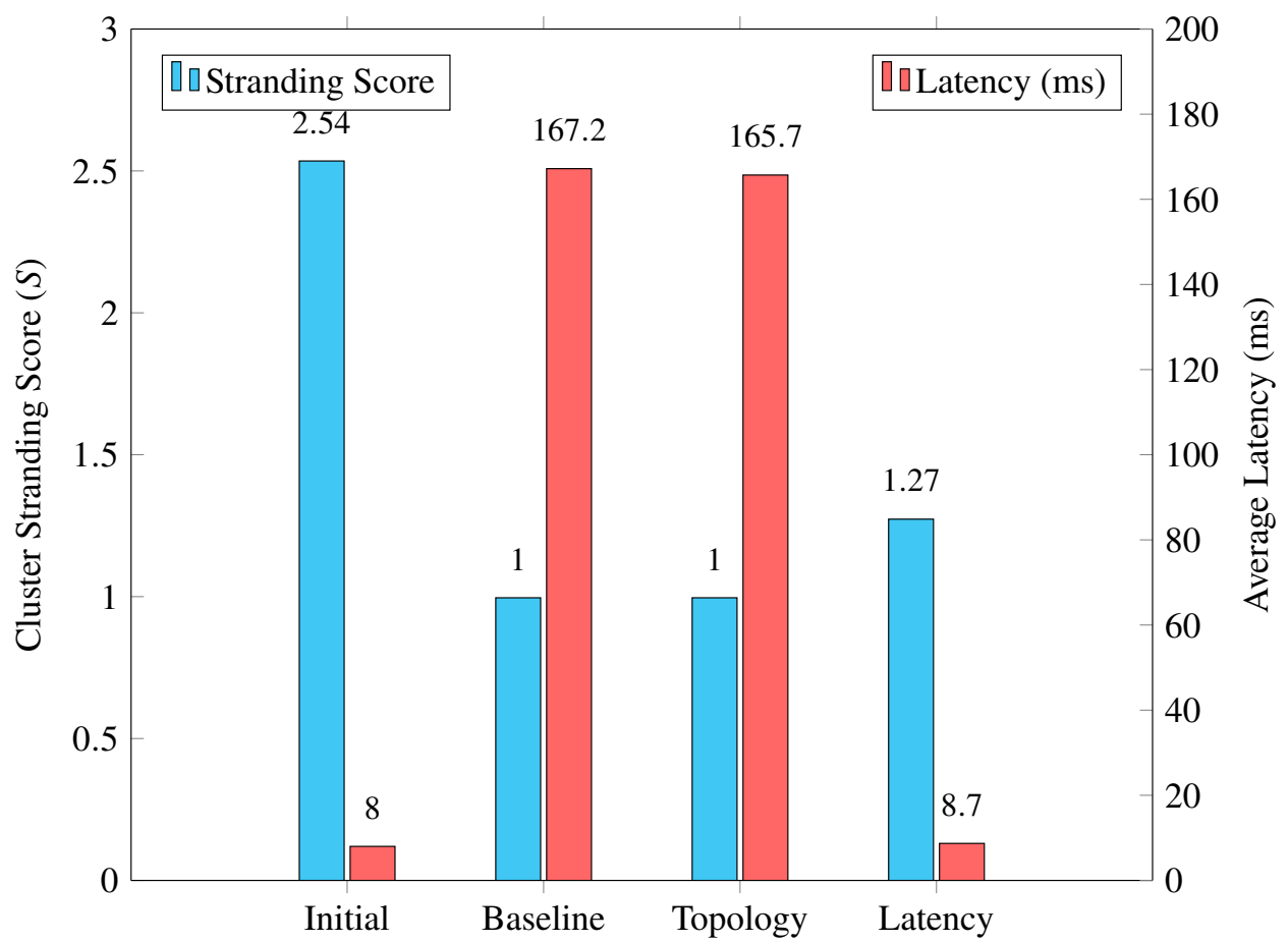
Figure 23. Cluster Stranding Score ( S ) vs. Network Performance.
