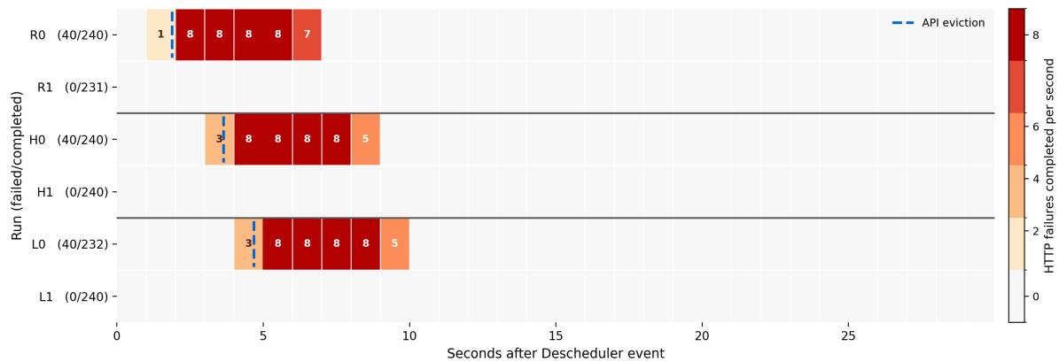
Figure 16. Event-Aligned HTTP Failure Timeline and API Eviction Time over the Common 30-Second Post-Event Window
