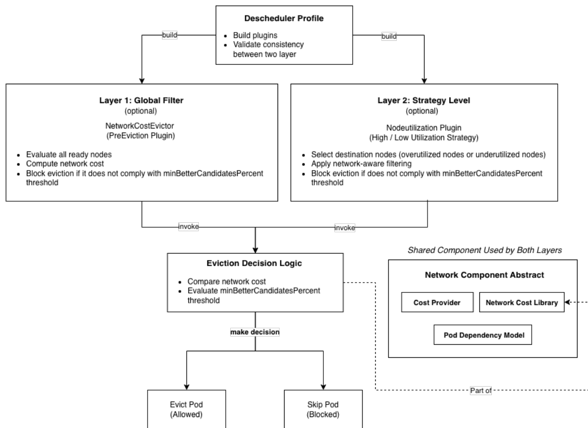
Figure 5. Network-Aware plugin architecture design.
