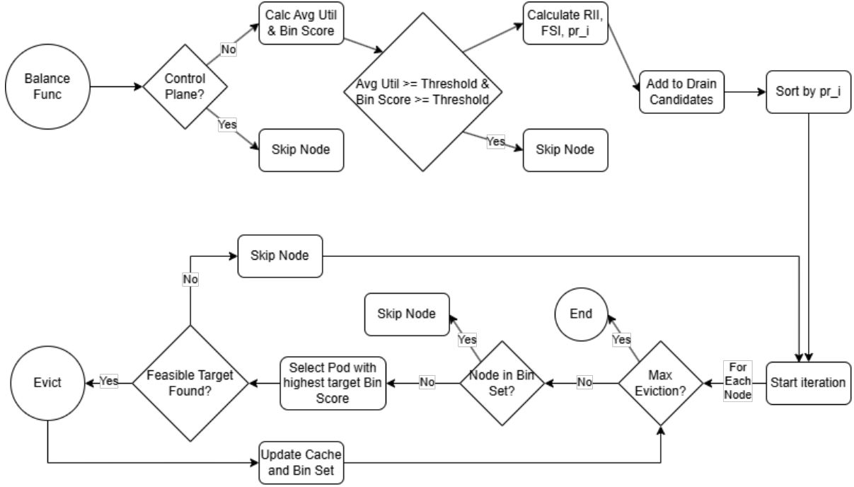
Figure 2. High-level control flow of the ResourceDefragmentation plugin, from Node assessment and drain-candidate ordering to the bounded predicted-target eviction loop.
