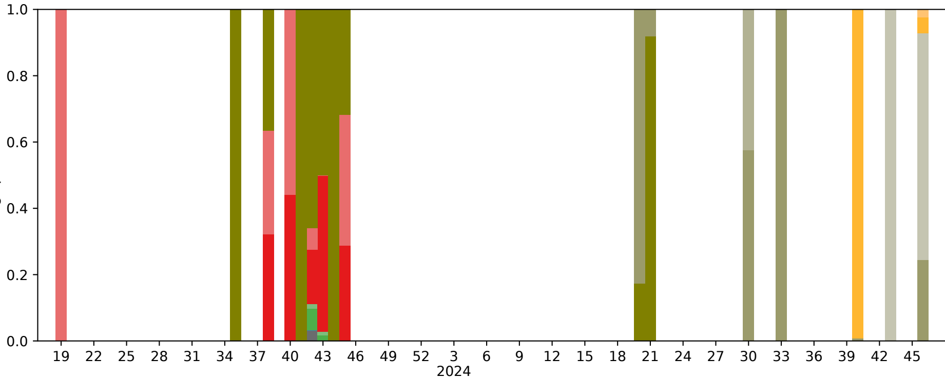
Lineage prevalence
