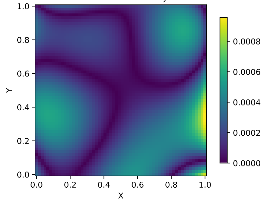
Normalized error u_y
