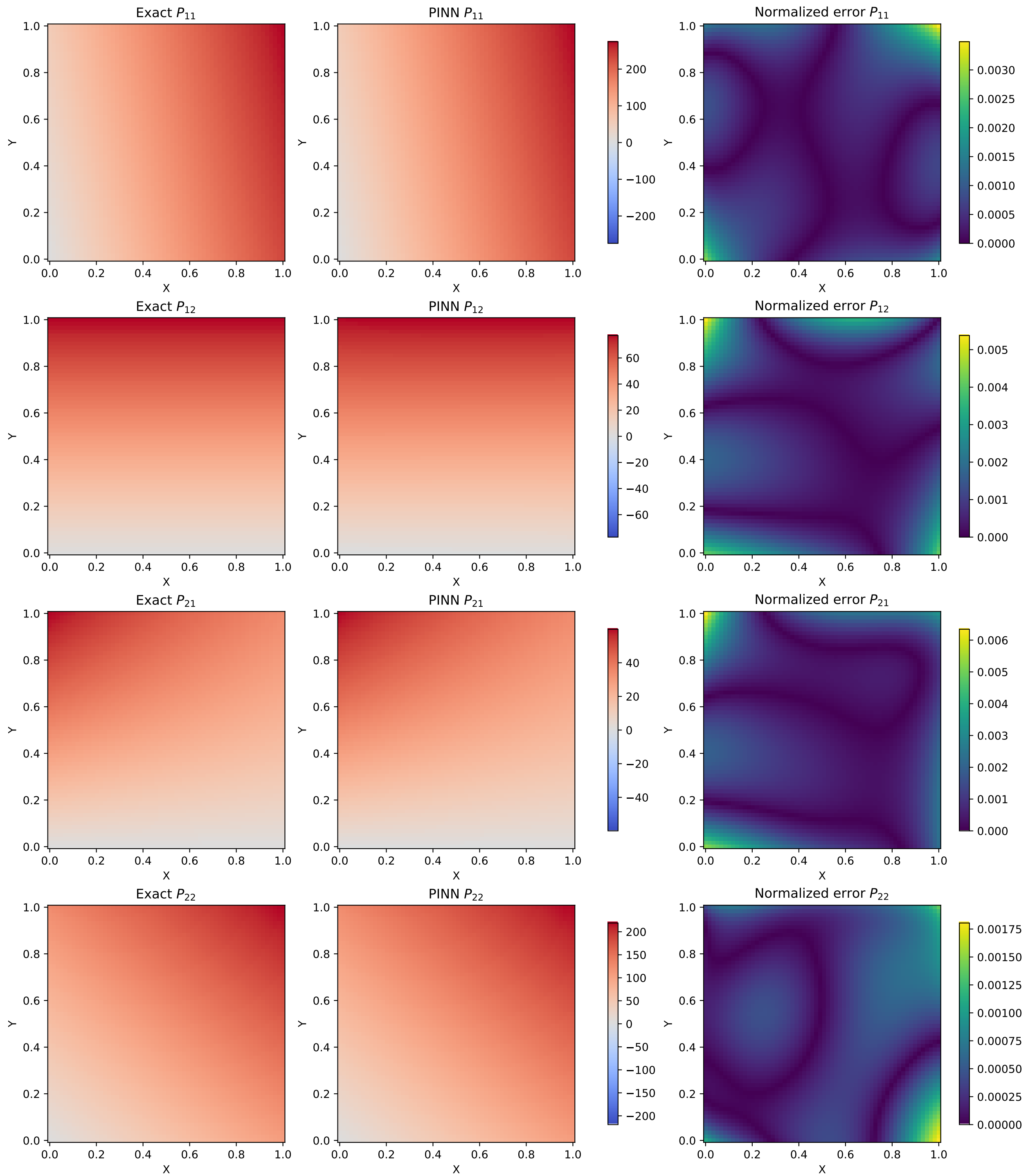
First Piola--Kirchhoff stress
