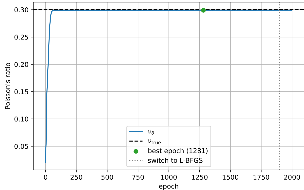
Identification of Poisson's ratio
