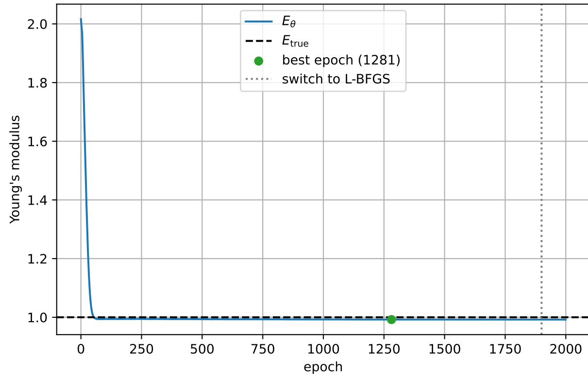
Identification of Young's modulus
