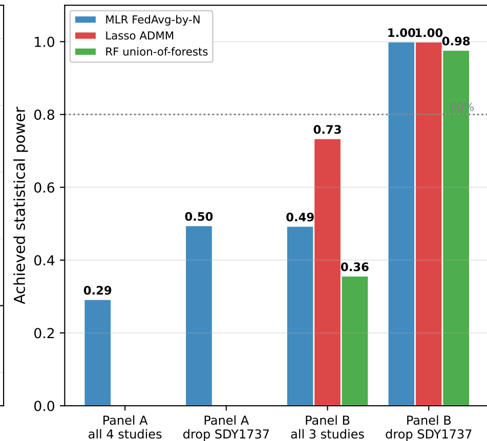
Federated post-Lasso pipeline: ADMM-Lasso selects features, MLR/Lasso/RF refit on the selection 5-fold stratified-by-Study CV • per-method aggregation (FedAvg-by-N for MLR, ADMM for Lasso, union of forests for RF)
