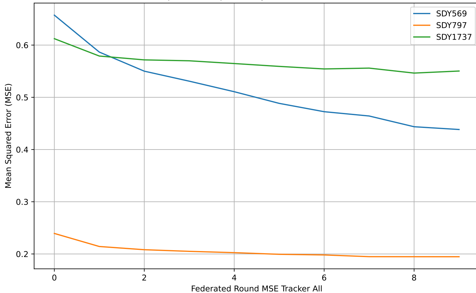
MSE per Round per Study — Federated CNN All
